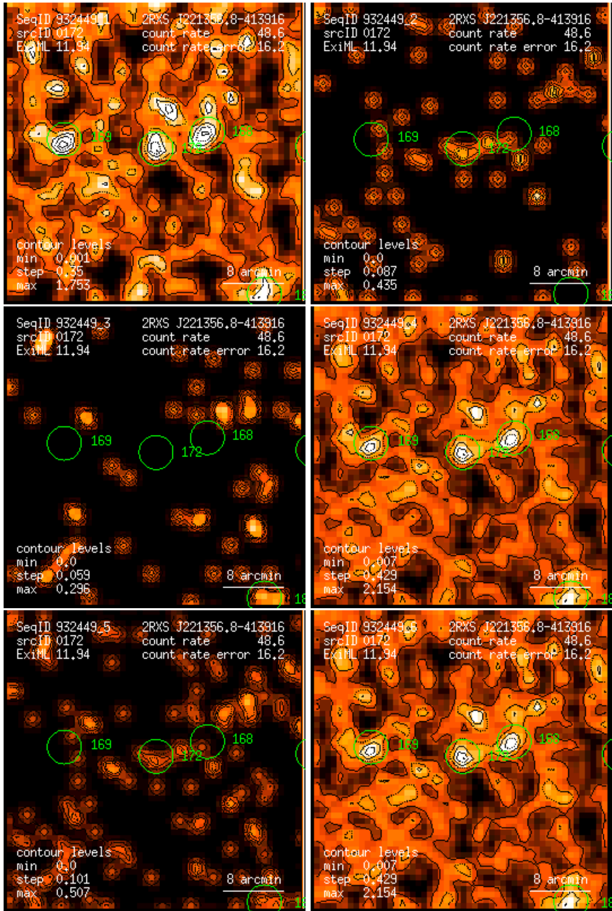
Figure 172: RASS 932449: detection 0172: band rate images, Gaussian filter: (1) PSPC channels 11 – 41, (2) 52 – 90, (3) 91 – 201, (4) 11 – 235, (5) 52 – 201, (6) 11 – 201. Broad band rates in counts/ks. Band rate contour levels in counts/ks/arcmin 2 .
