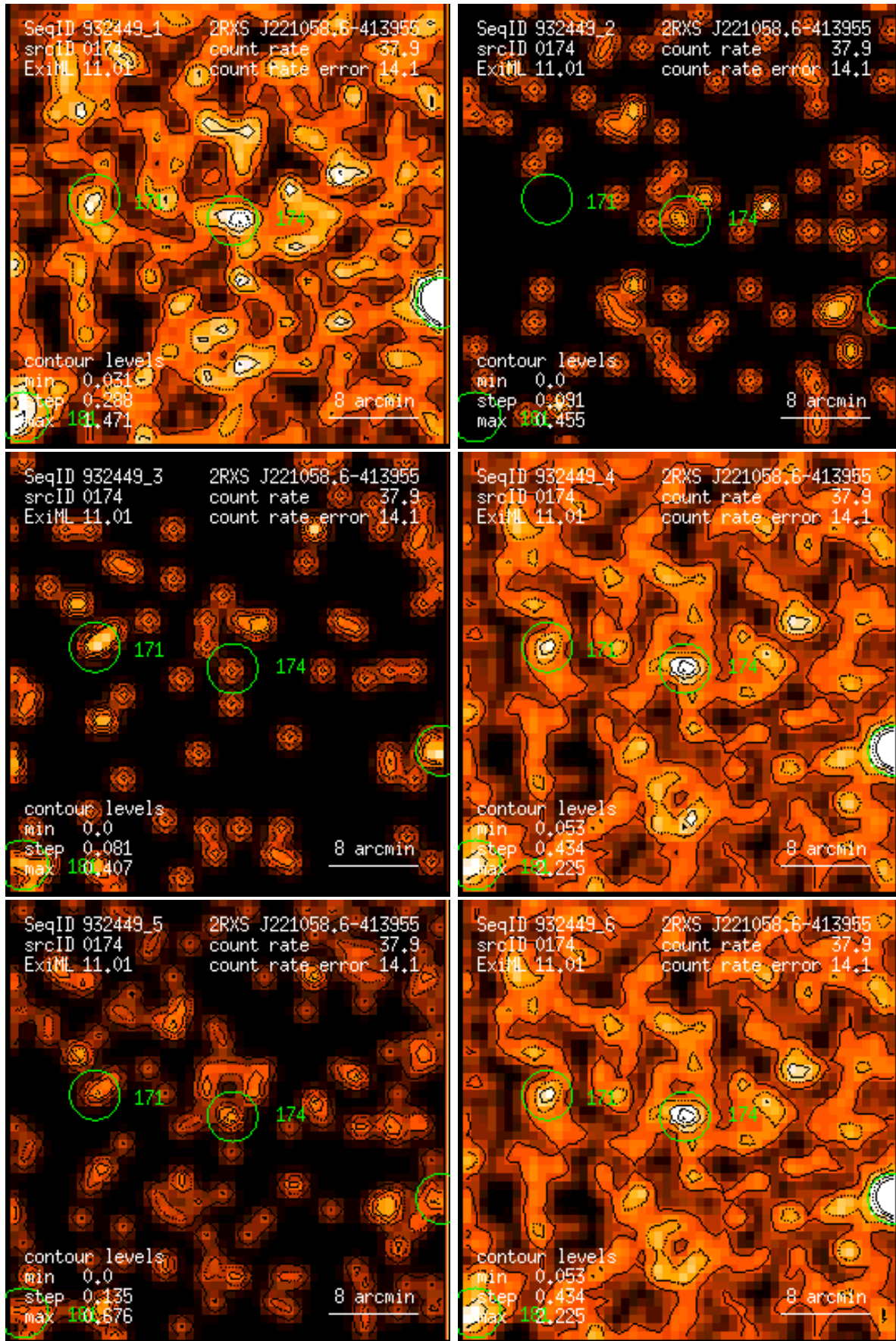
Figure 174: RASS 932449: detection 0174: band rate images, Gaussian filter: (1) PSPC channels 11 – 41, (2) 52 – 90, (3) 91 – 201, (4) 11 – 235, (5) 52 – 201, (6) 11 – 201. Broad band rates in counts/ks. Band rate contour levels in counts/ks/arcmin 2 .
