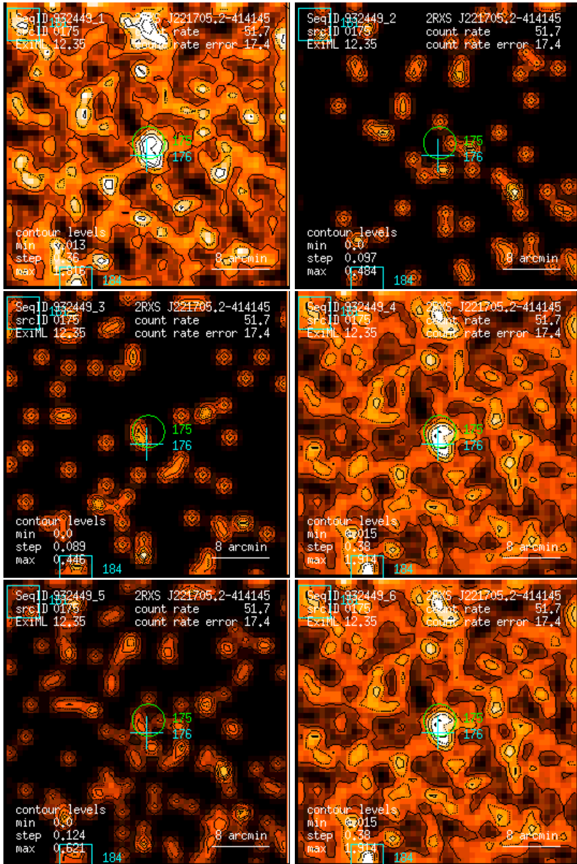
Figure 175: RASS 932449: detection 0175: band rate images, Gaussian filter: (1) PSPC channels 11 – 41, (2) 52 – 90, (3) 91 – 201, (4) 11 – 235, (5) 52 – 201, (6) 11 – 201. Broad band rates in counts/ks. Band rate contour levels in counts/ks/arcmin 2 .
