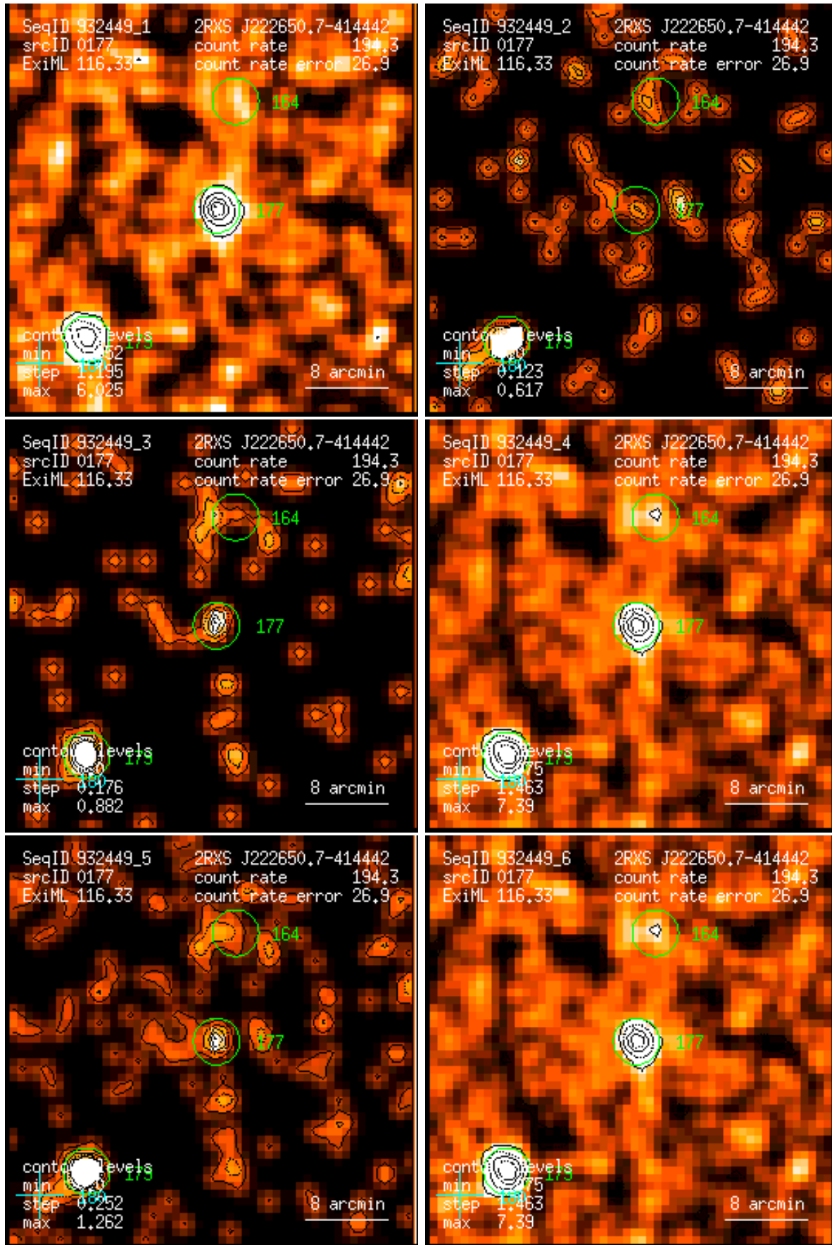
Figure 177: RASS 932449: detection 0177: band rate images, Gaussian filter: (1) PSPC channels 11 – 41, (2) 52 – 90, (3) 91 – 201, (4) 11 – 235, (5) 52 – 201, (6) 11 – 201. Broad band rates in counts/ks. Band rate contour levels in counts/ks/arcmin 2 .
