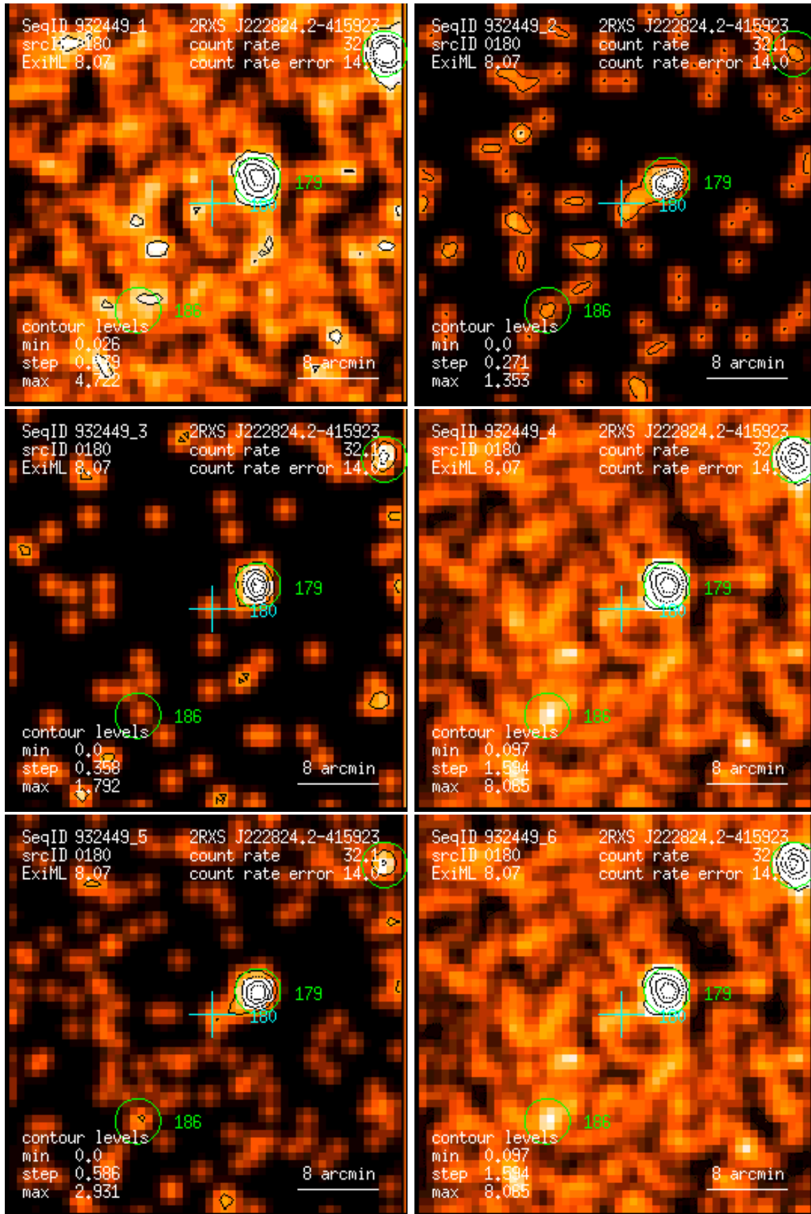
Figure 180: RASS 932449: detection 0180: band rate images, Gaussian filter: (1) PSPC channels 11 – 41, (2) 52 – 90, (3) 91 – 201, (4) 11 – 235, (5) 52 – 201, (6) 11 – 201. Broad band rates in counts/ks. Band rate contour levels in counts/ks/arcmin 2 .
