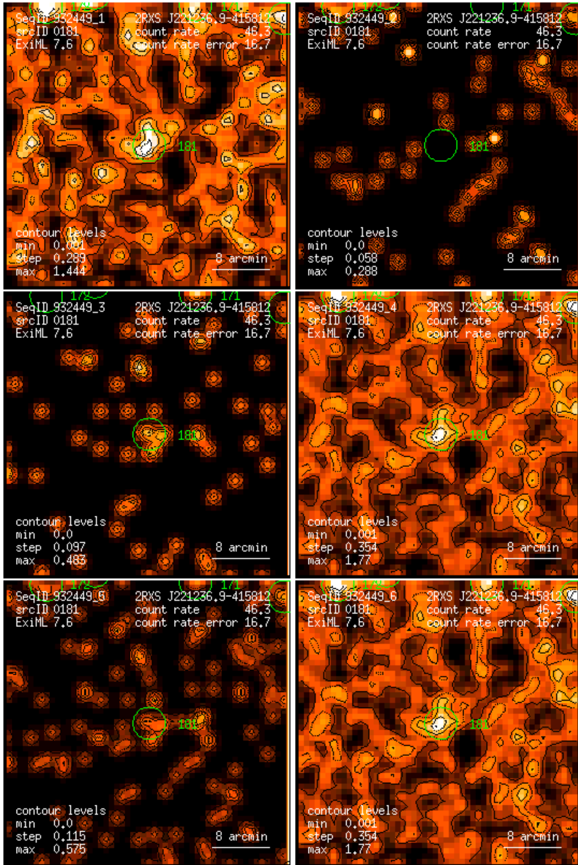
Figure 181: RASS 932449: detection 0181: band rate images, Gaussian filter: (1) PSPC channels 11 – 41, (2) 52 – 90, (3) 91 – 201, (4) 11 – 235, (5) 52 – 201, (6) 11 – 201. Broad band rates in counts/ks. Band rate contour levels in counts/ks/arcmin 2 .
