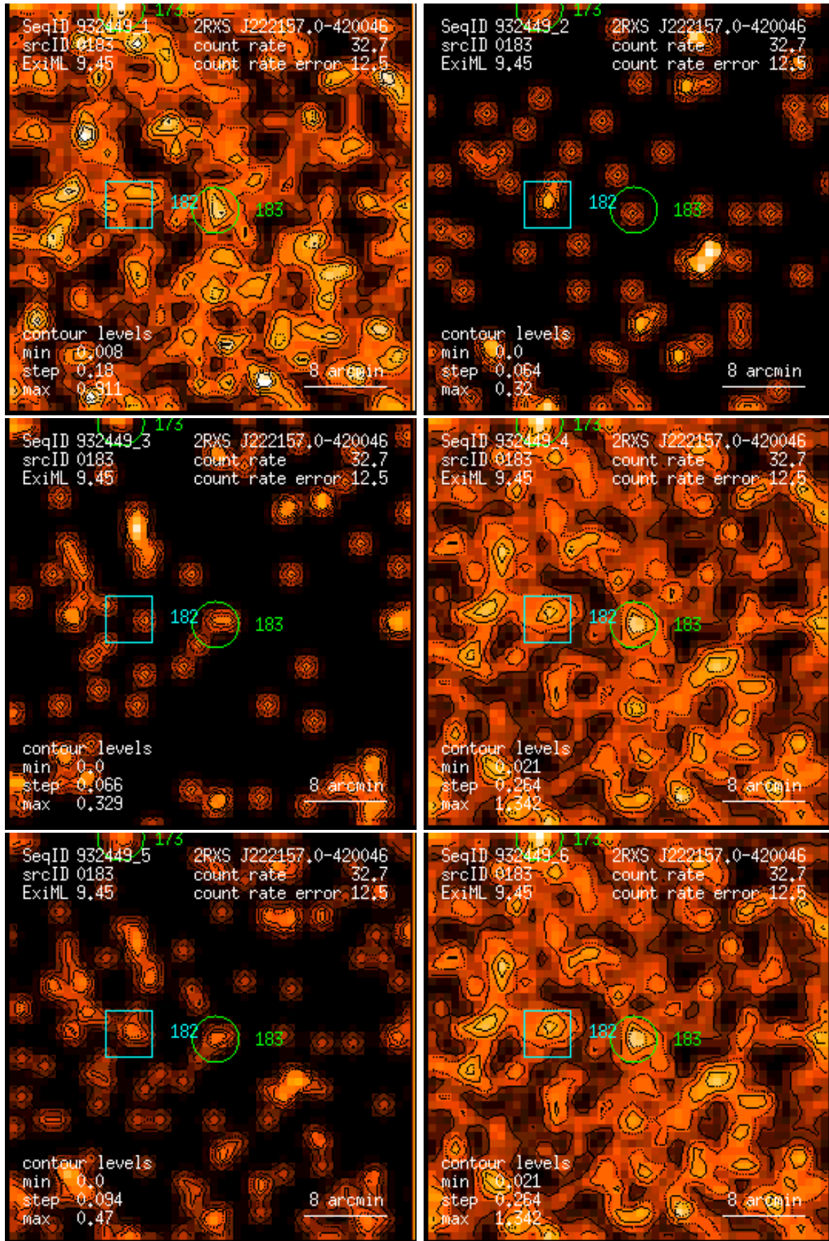
Figure 183: RASS 932449: detection 0183: band rate images, Gaussian filter: (1) PSPC channels 11 – 41, (2) 52 – 90, (3) 91 – 201, (4) 11 – 235, (5) 52 – 201, (6) 11 – 201. Broad band rates in counts/ks. Band rate contour levels in counts/ks/arcmin 2 .
