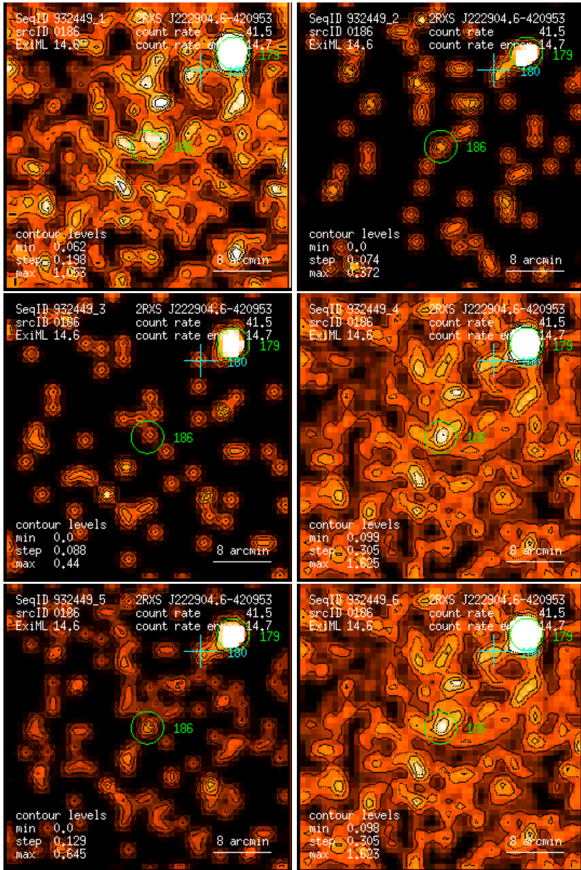
Figure 186: RASS 932449: detection 0186: band rate images, Gaussian filter: (1) PSPC channels 11 – 41, (2) 52 – 90, (3) 91 – 201, (4) 11 – 235, (5) 52 – 201, (6) 11 – 201. Broad band rates in counts/ks. Band rate contour levels in counts/ks/arcmin 2 .
