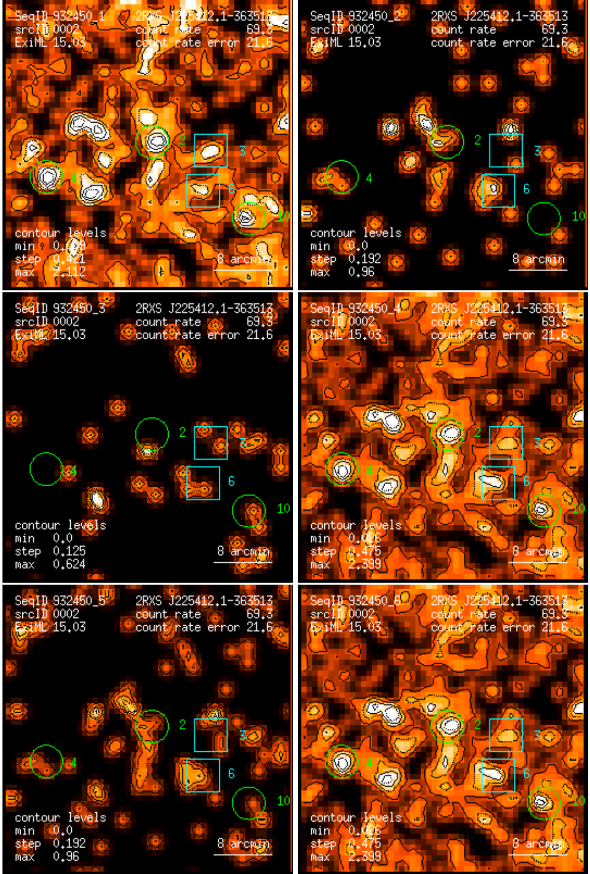
Figure 2: RASS 932450: detection 0002: band rate images, Gaussian filter: (1) PSPC channels 11 – 41, (2) 52 – 90, (3) 91 – 201, (4) 11 – 235, (5) 52 – 201, (6) 11 – 201. Broad band rates in counts/ks. Band rate contour levels in counts/ks/arcmin 2 .
