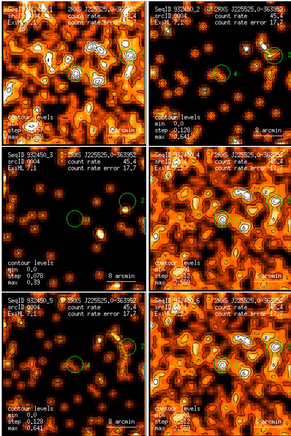
Figure 4: RASS 932450: detection 0004: band rate images, Gaussian filter: (1) PSPC channels 11 – 41, (2) 52 – 90, (3) 91 – 201, (4) 11 – 235, (5) 52 – 201, (6) 11 – 201. Broad band rates in counts/ks. Band rate contour levels in counts/ks/arcmin 2 .
