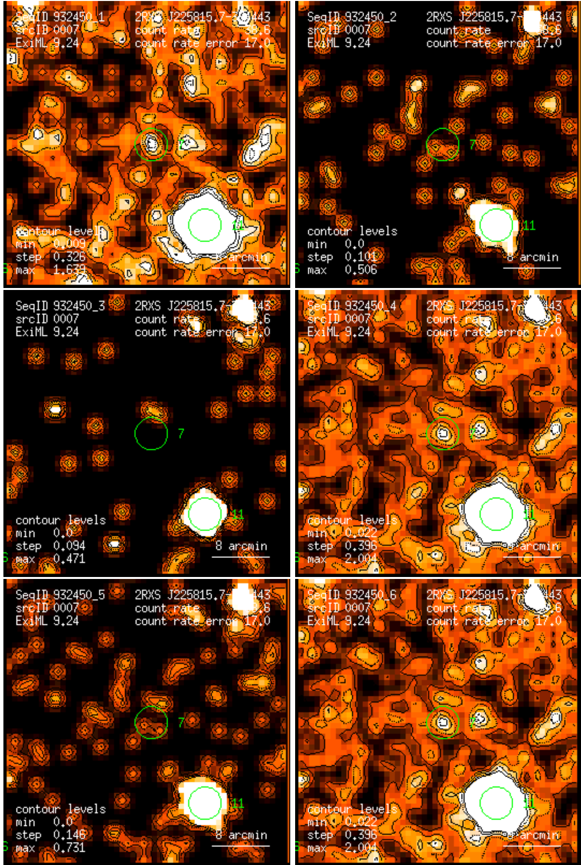
Figure 7: RASS 932450: detection 0007: band rate images, Gaussian filter: (1) PSPC channels 11 – 41, (2) 52 – 90, (3) 91 – 201, (4) 11 – 235, (5) 52 – 201, (6) 11 – 201. Broad band rates in counts/ks. Band rate contour levels in counts/ks/arcmin 2 .
