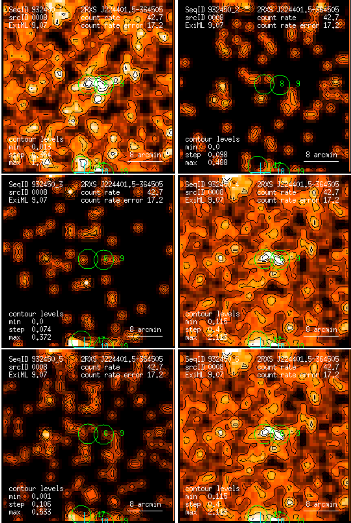
Figure 8: RASS 932450: detection 0008: band rate images, Gaussian filter: (1) PSPC channels 11 – 41, (2) 52 – 90, (3) 91 – 201, (4) 11 – 235, (5) 52 – 201, (6) 11 – 201. Broad band rates in counts/ks. Band rate contour levels in counts/ks/arcmin 2 .
