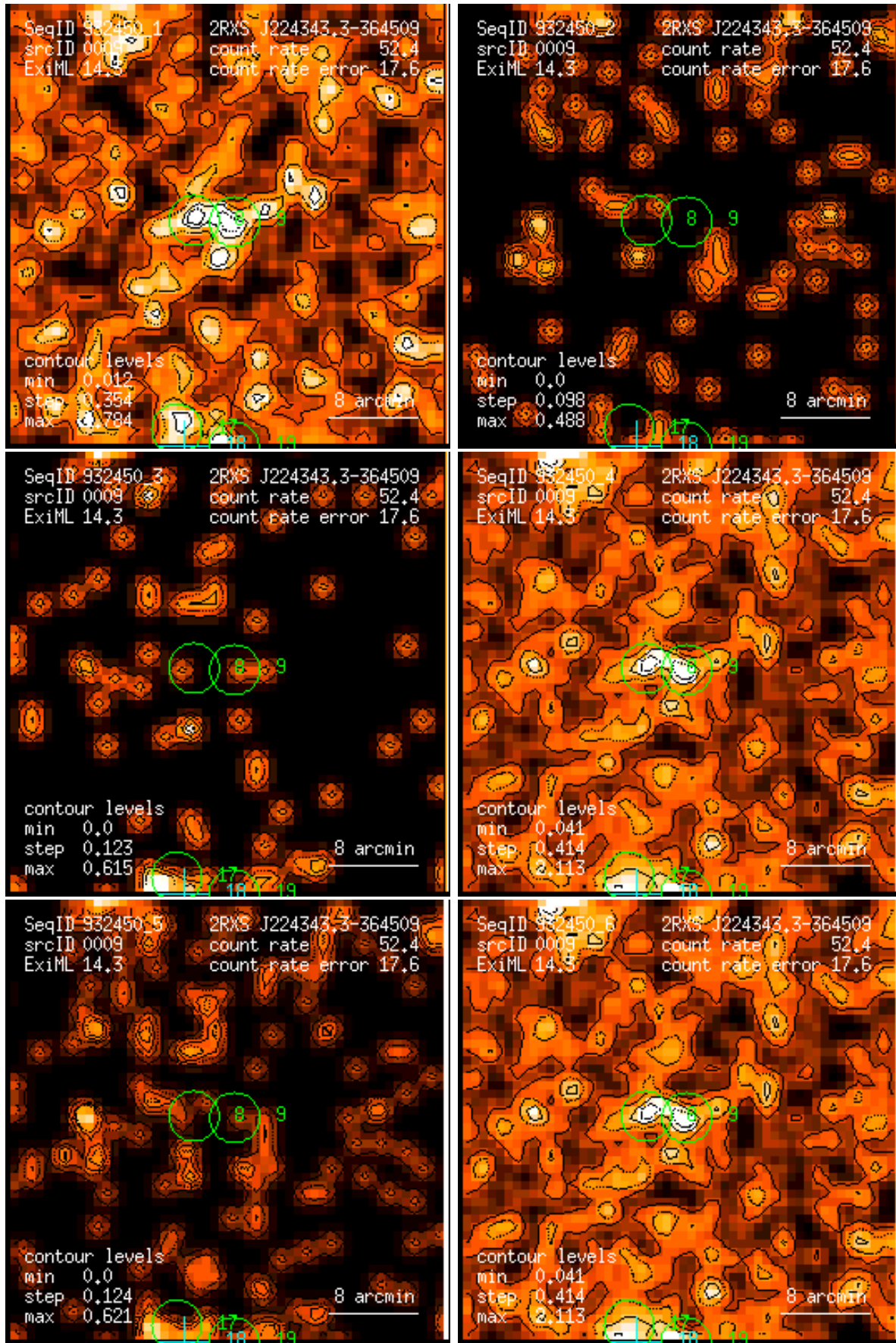
Figure 9: RASS 932450: detection 0009: band rate images, Gaussian filter: (1) PSPC channels 11 – 41, (2) 52 – 90, (3) 91 – 201, (4) 11 – 235, (5) 52 – 201, (6) 11 – 201. Broad band rates in counts/ks. Band rate contour levels in counts/ks/arcmin 2 .
