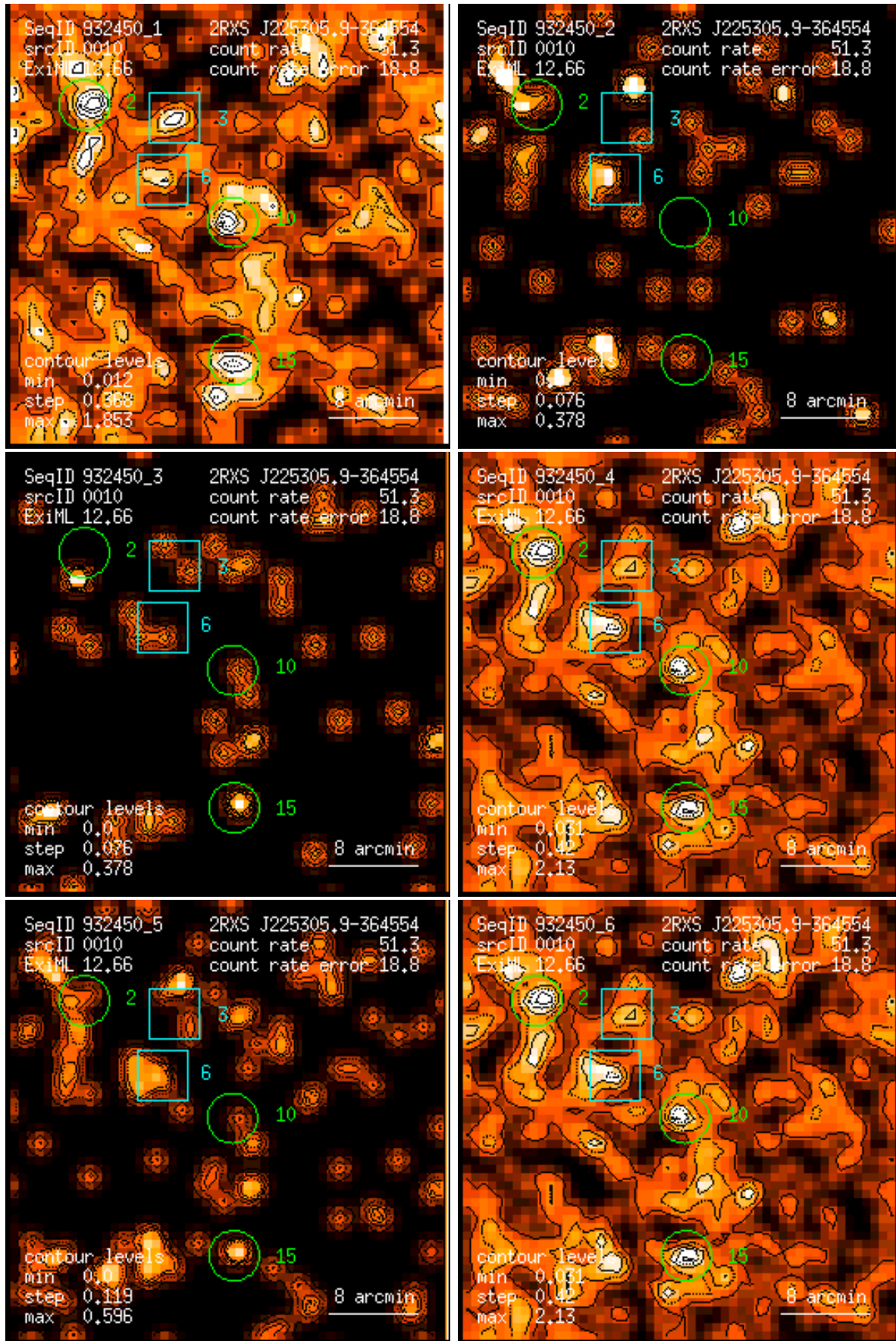
Figure 10: RASS 932450: detection 0010: band rate images, Gaussian filter: (1) PSPC channels 11 – 41, (2) 52 – 90, (3) 91 – 201, (4) 11 – 235, (5) 52 – 201, (6) 11 – 201. Broad band rates in counts/ks. Band rate contour levels in counts/ks/arcmin 2 .
