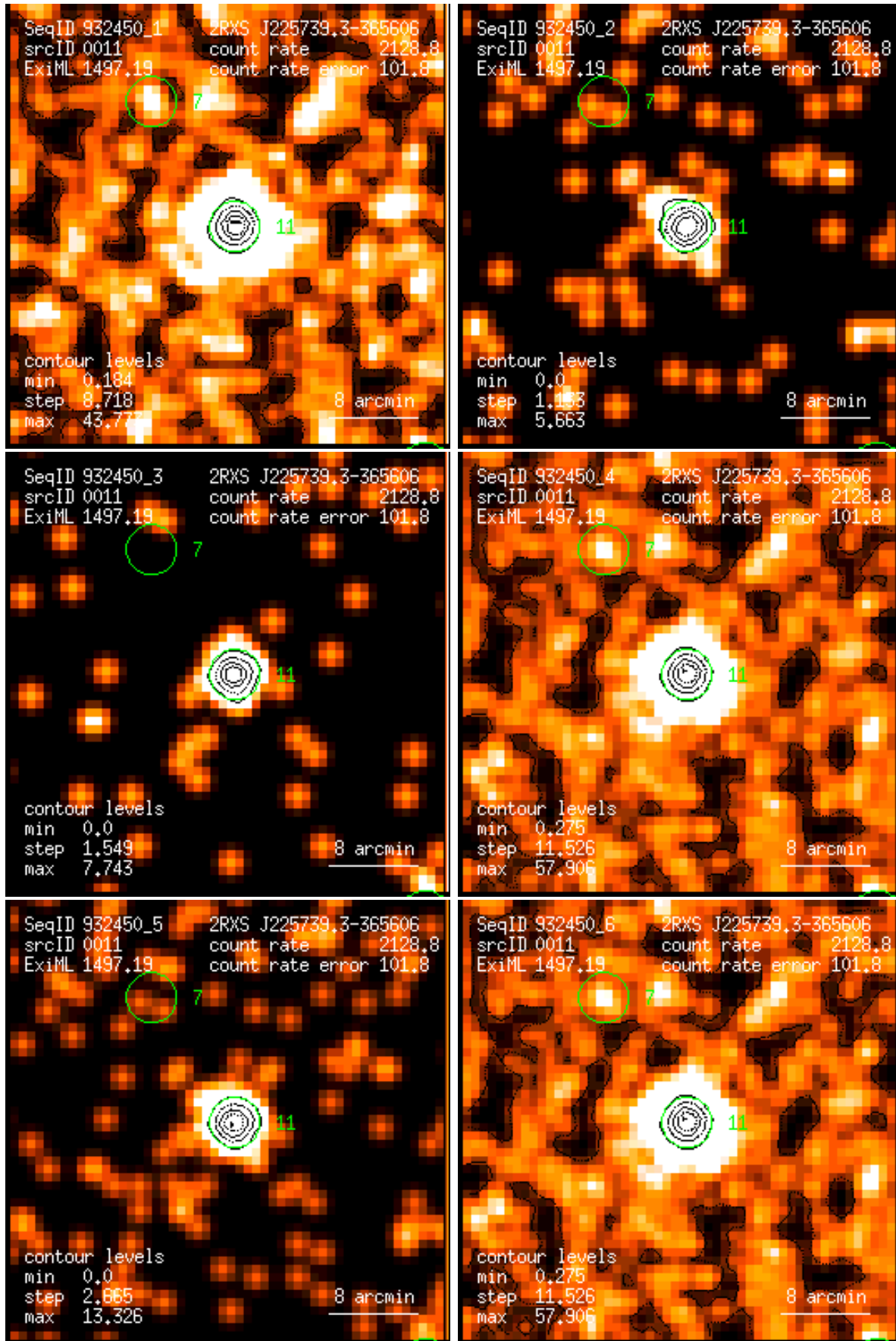
Figure 11: RASS 932450: detection 0011: band rate images, Gaussian filter: (1) PSPC channels 11 – 41, (2) 52 – 90, (3) 91 – 201, (4) 11 – 235, (5) 52 – 201, (6) 11 – 201. Broad band rates in counts/ks. Band rate contour levels in counts/ks/arcmin 2 .
