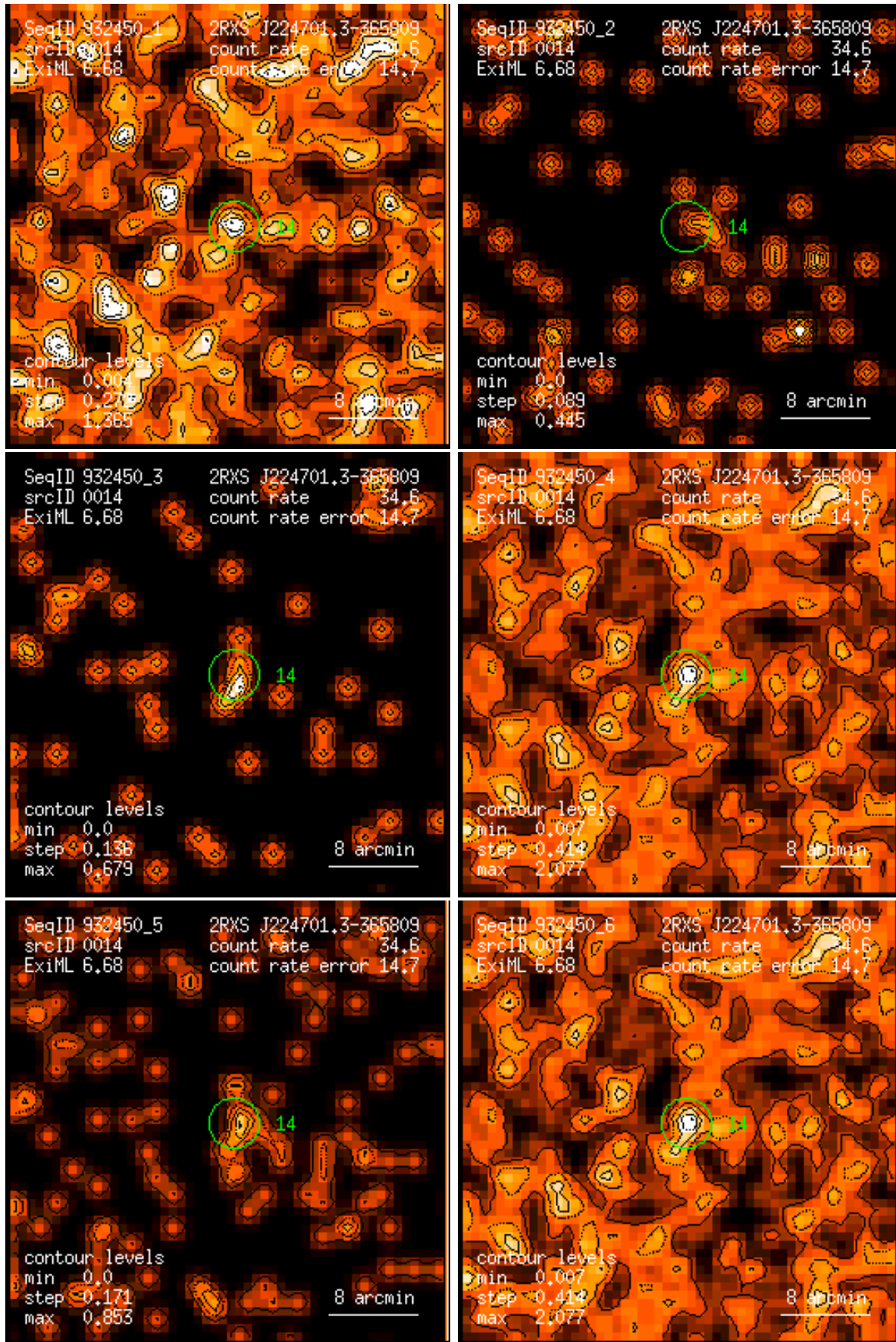
Figure 14: RASS 932450: detection 0014: band rate images, Gaussian filter: (1) PSPC channels 11 – 41, (2) 52 – 90, (3) 91 – 201, (4) 11 – 235, (5) 52 – 201, (6) 11 – 201. Broad band rates in counts/ks. Band rate contour levels in counts/ks/arcmin 2 .
