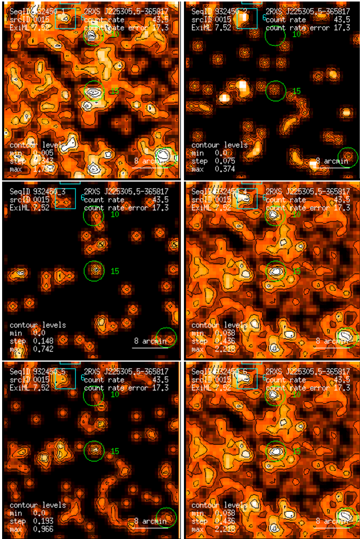
Figure 15: RASS 932450: detection 0015: band rate images, Gaussian filter: (1) PSPC channels 11 – 41, (2) 52 – 90, (3) 91 – 201, (4) 11 – 235, (5) 52 – 201, (6) 11 – 201. Broad band rates in counts/ks. Band rate contour levels in counts/ks/arcmin 2 .
