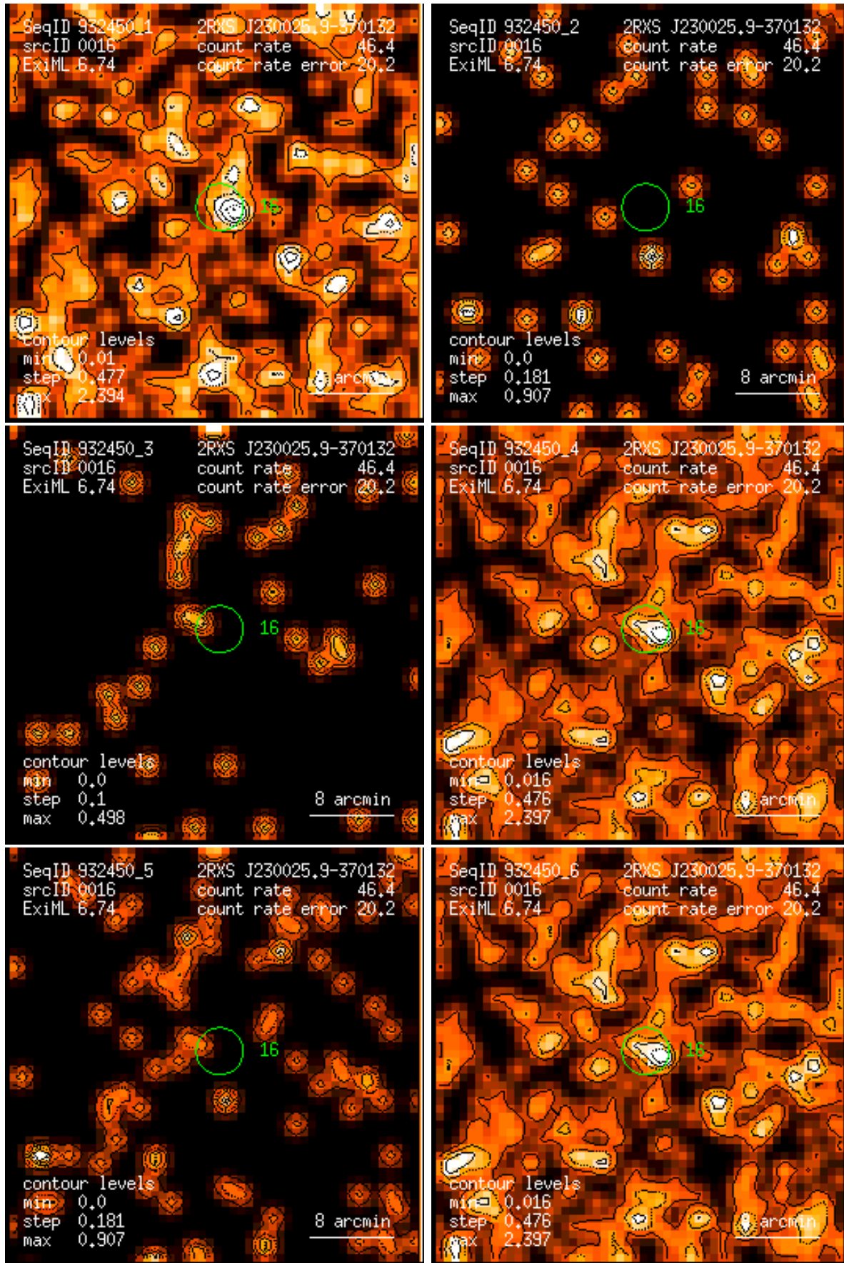
Figure 16: RASS 932450: detection 0016: band rate images, Gaussian filter: (1) PSPC channels 11 – 41, (2) 52 – 90, (3) 91 – 201, (4) 11 – 235, (5) 52 – 201, (6) 11 – 201. Broad band rates in counts/ks. Band rate contour levels in counts/ks/arcmin 2 .
