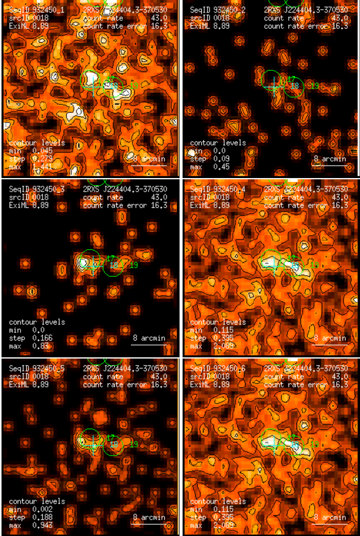
Figure 18: RASS 932450: detection 0018: band rate images, Gaussian filter: (1) PSPC channels 11 – 41, (2) 52 – 90, (3) 91 – 201, (4) 11 – 235, (5) 52 – 201, (6) 11 – 201. Broad band rates in counts/ks. Band rate contour levels in counts/ks/arcmin 2 .
