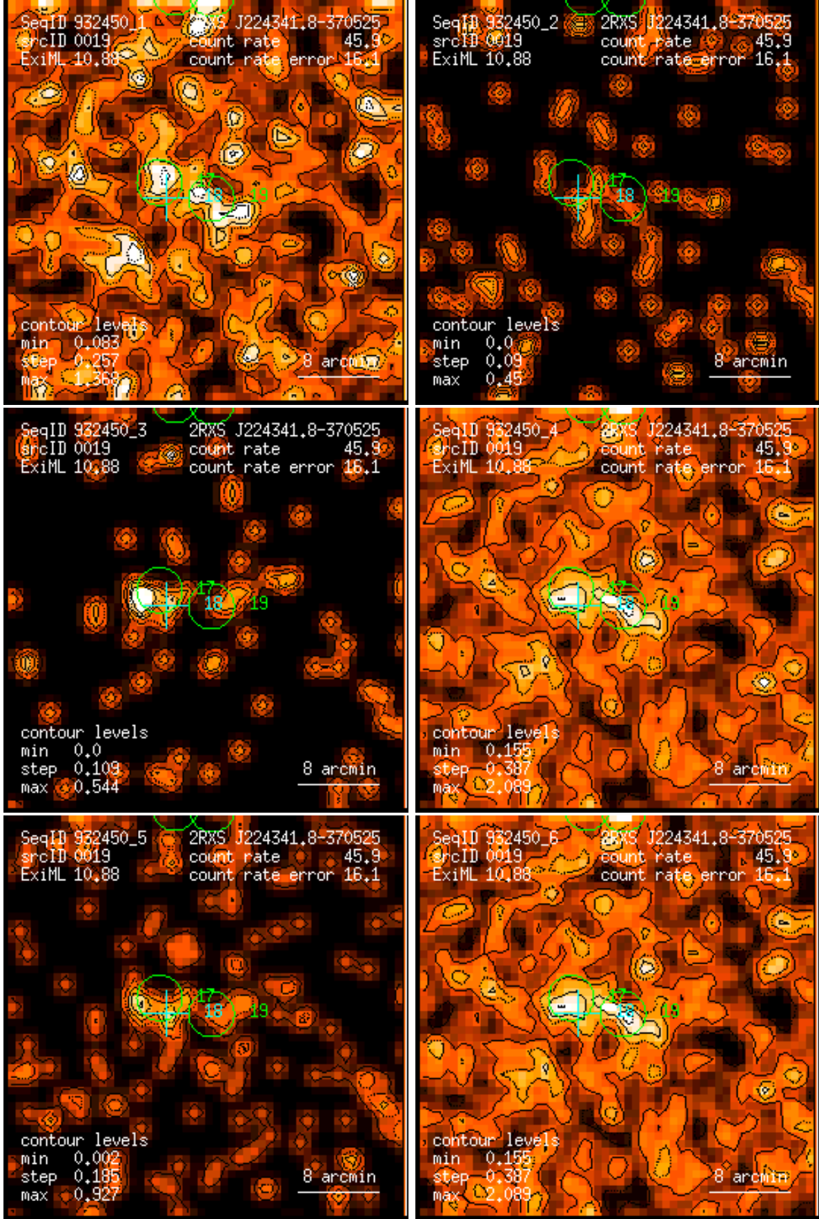
Figure 19: RASS 932450: detection 0019: band rate images, Gaussian filter: (1) PSPC channels 11 – 41, (2) 52 – 90, (3) 91 – 201, (4) 11 – 235, (5) 52 – 201, (6) 11 – 201. Broad band rates in counts/ks. Band rate contour levels in counts/ks/arcmin 2 .
