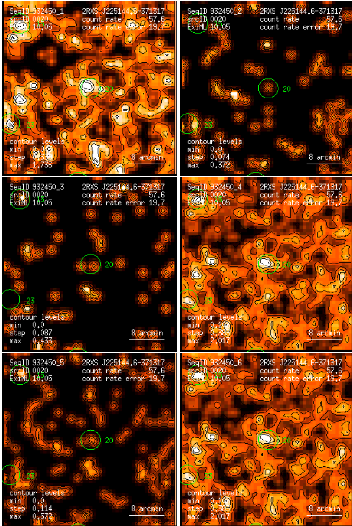
Figure 20: RASS 932450: detection 0020: band rate images, Gaussian filter: (1) PSPC channels 11 – 41, (2) 52 – 90, (3) 91 – 201, (4) 11 – 235, (5) 52 – 201, (6) 11 – 201. Broad band rates in counts/ks. Band rate contour levels in counts/ks/arcmin 2 .
