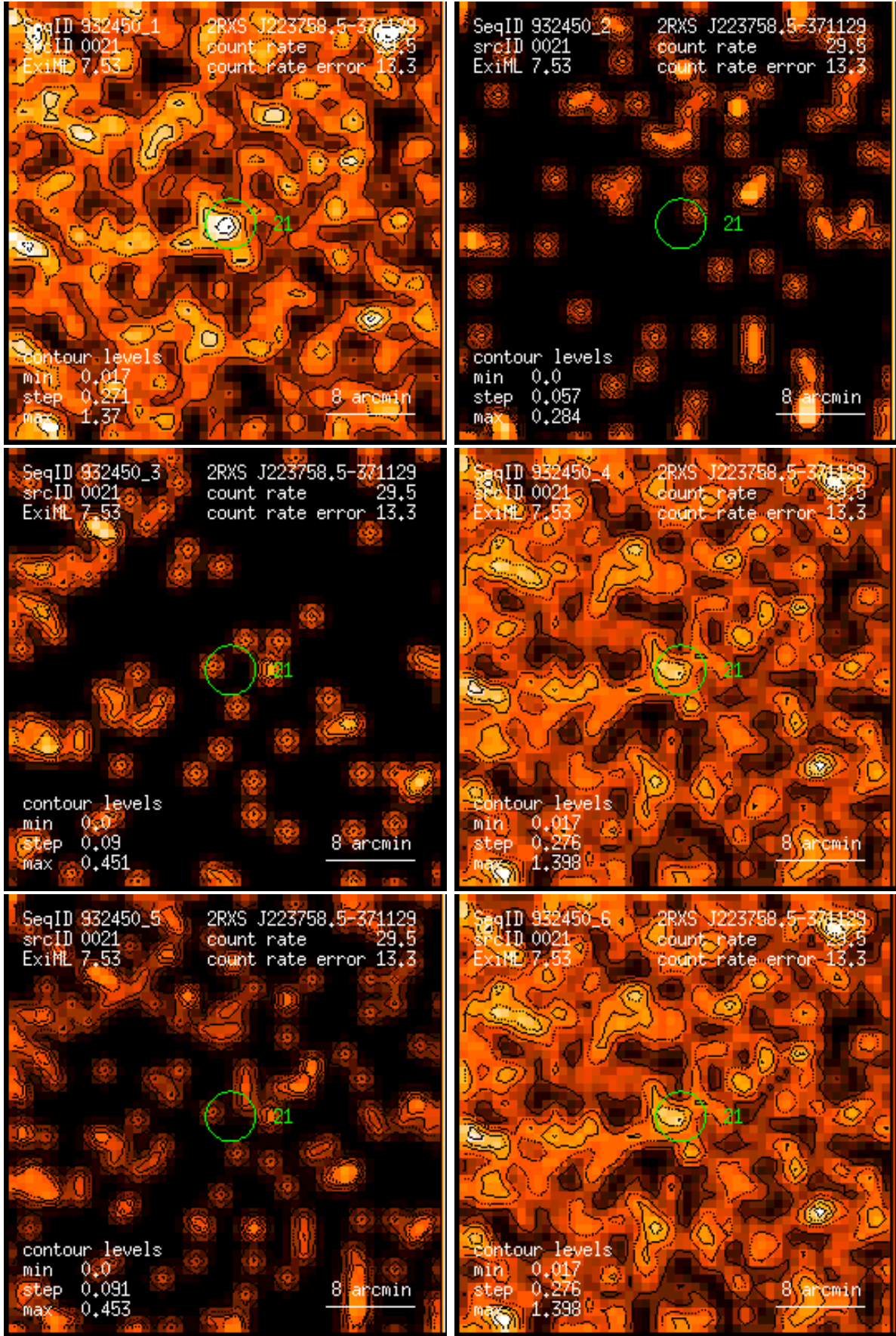
Figure 21: RASS 932450: detection 0021: band rate images, Gaussian filter: (1) PSPC channels 11 – 41, (2) 52 – 90, (3) 91 – 201, (4) 11 – 235, (5) 52 – 201, (6) 11 – 201. Broad band rates in counts/ks. Band rate contour levels in counts/ks/arcmin 2 .
