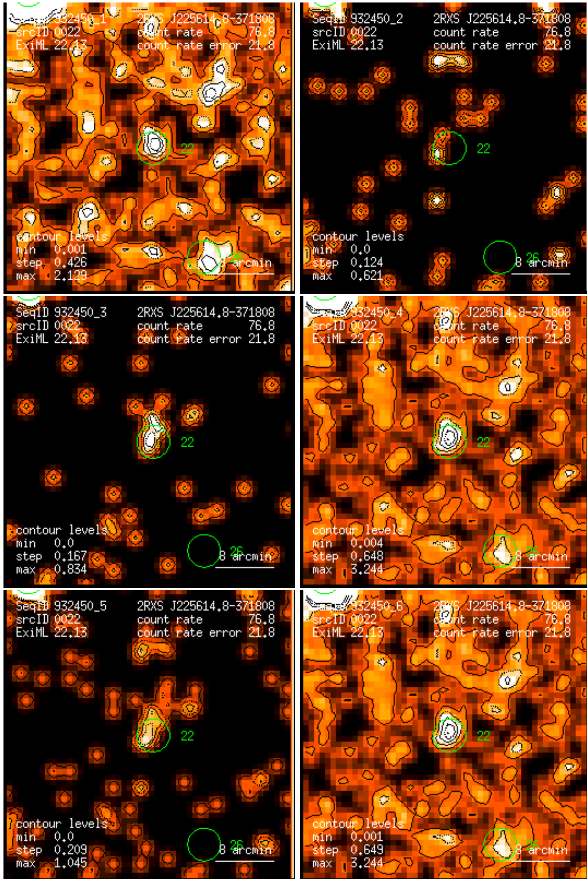
Figure 22: RASS 932450: detection 0022: band rate images, Gaussian filter: (1) PSPC channels 11 – 41, (2) 52 – 90, (3) 91 – 201, (4) 11 – 235, (5) 52 – 201, (6) 11 – 201. Broad band rates in counts/ks. Band rate contour levels in counts/ks/arcmin 2 .
