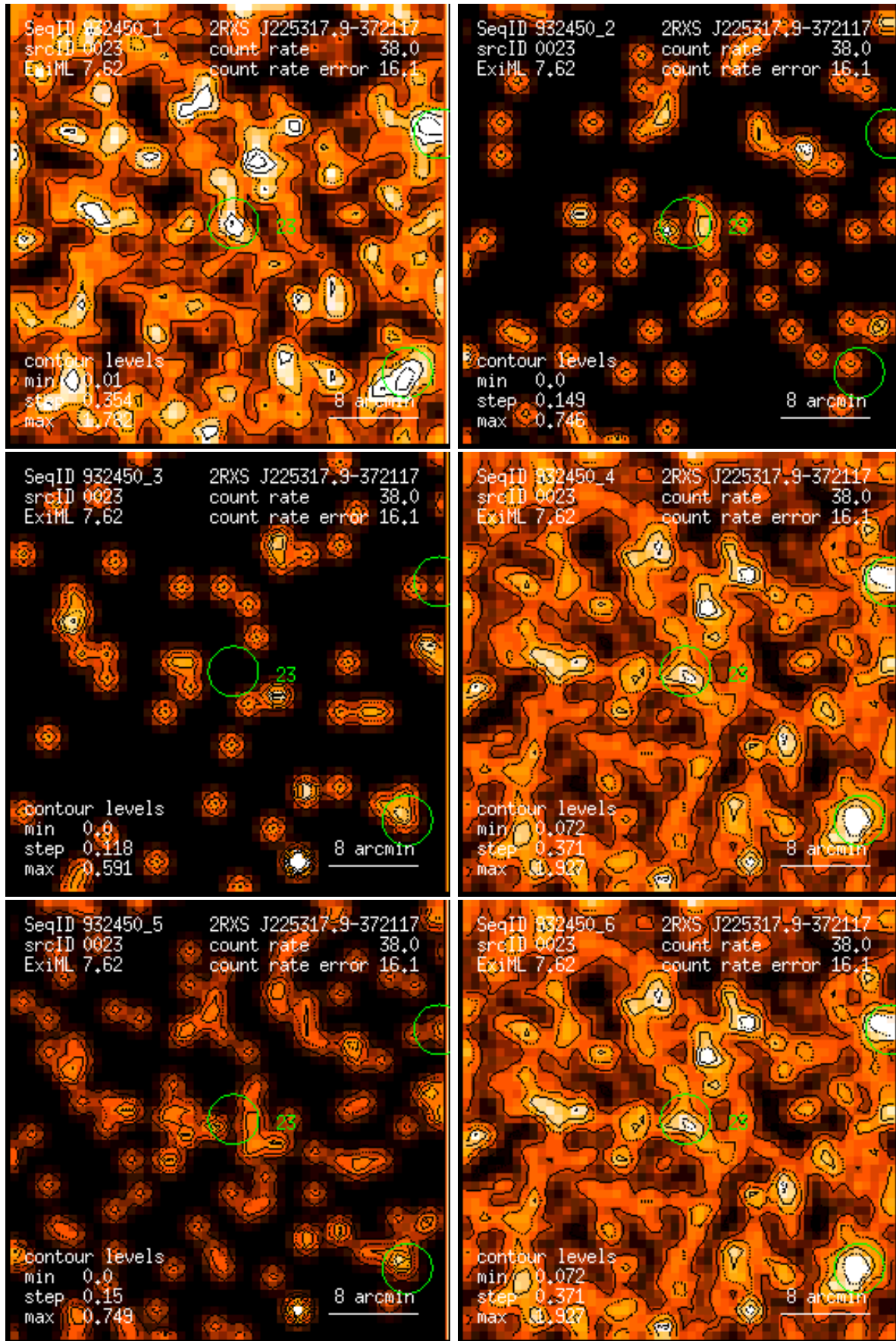
Figure 23: RASS 932450: detection 0023: band rate images, Gaussian filter: (1) PSPC channels 11 – 41, (2) 52 – 90, (3) 91 – 201, (4) 11 – 235, (5) 52 – 201, (6) 11 – 201. Broad band rates in counts/ks. Band rate contour levels in counts/ks/arcmin 2 .
