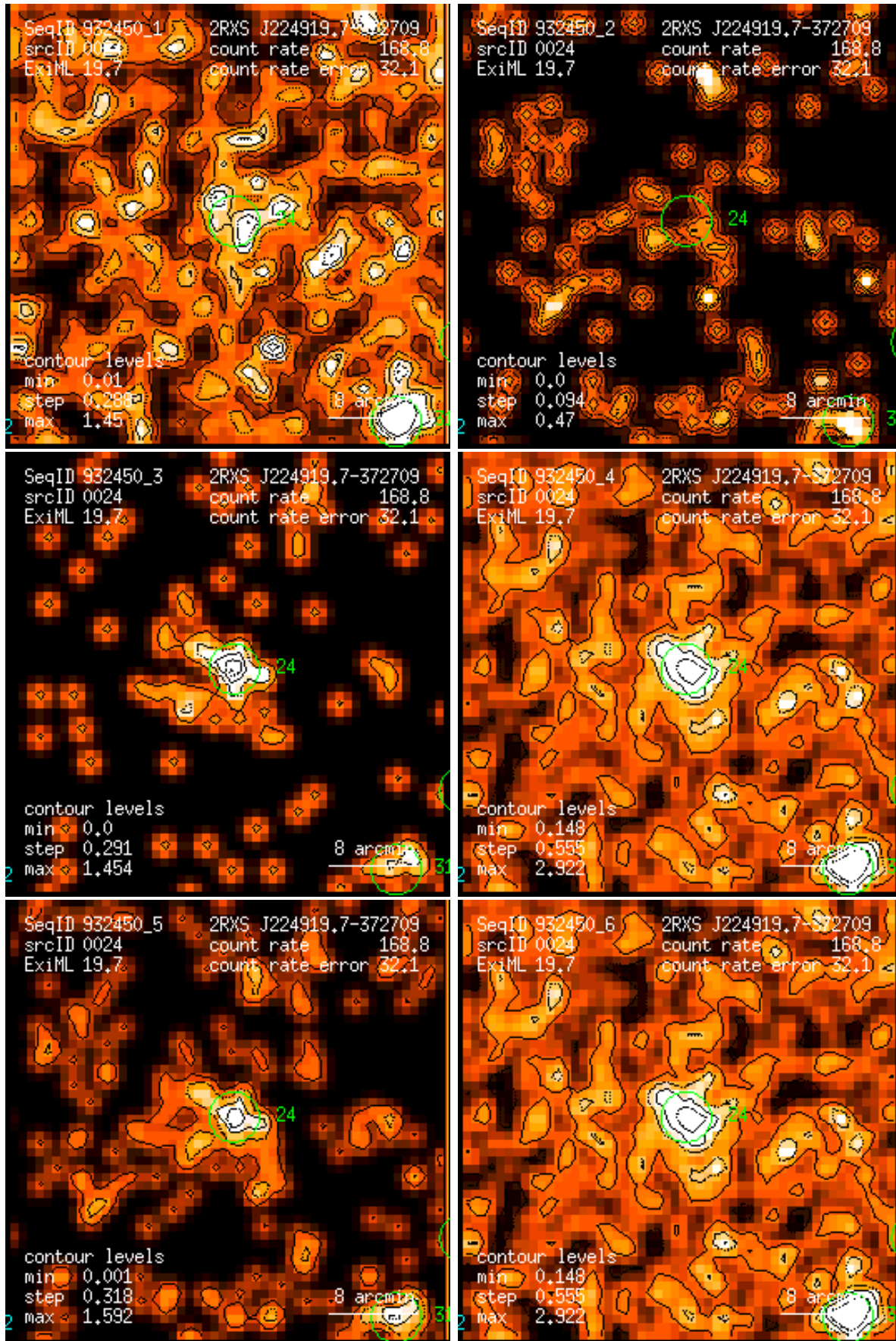
Figure 24: RASS 932450: detection 0024: band rate images, Gaussian filter: (1) PSPC channels 11 – 41, (2) 52 – 90, (3) 91 – 201, (4) 11 – 235, (5) 52 – 201, (6) 11 – 201. Broad band rates in counts/ks. Band rate contour levels in counts/ks/arcmin 2 .
