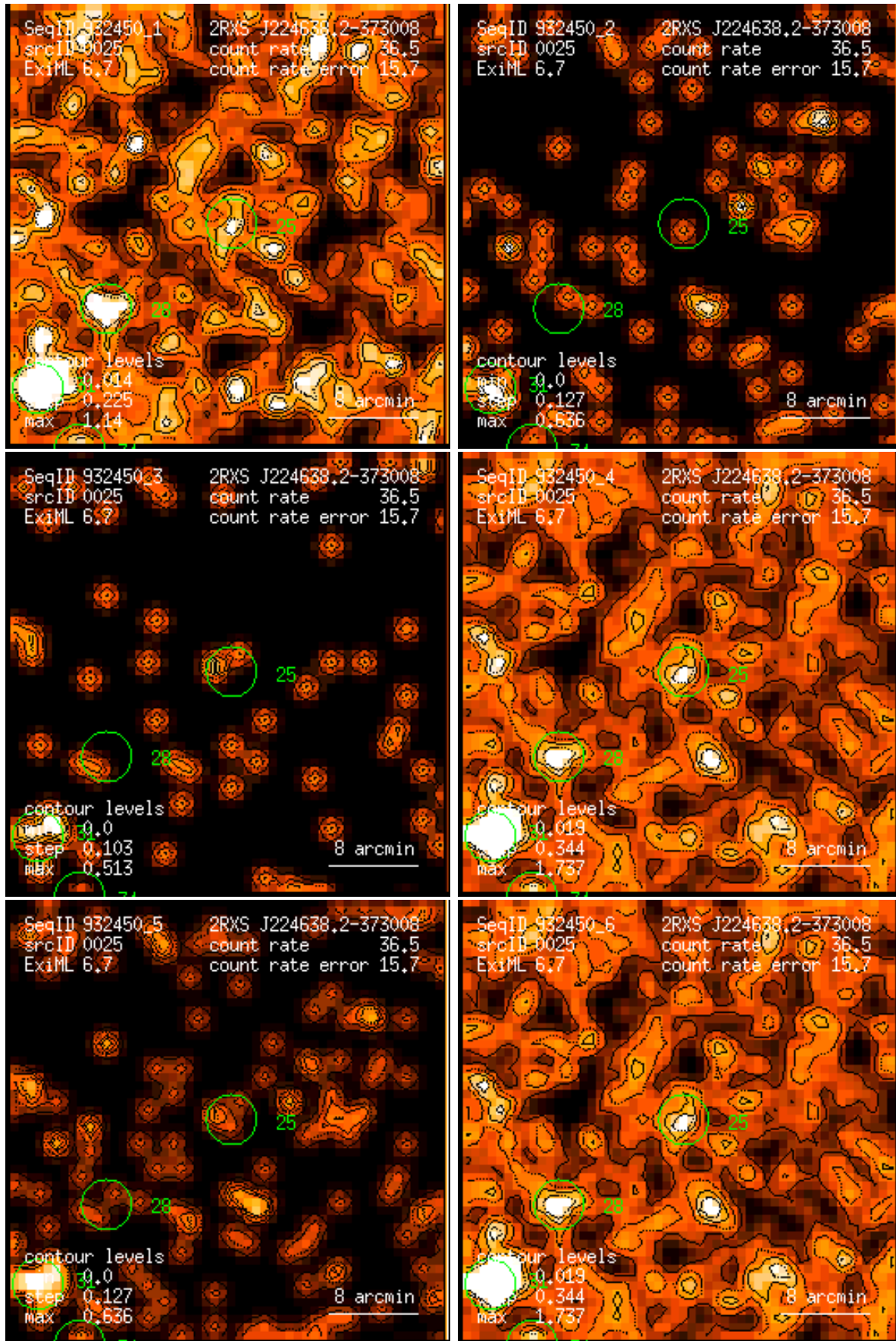
Figure 25: RASS 932450: detection 0025: band rate images, Gaussian filter: (1) PSPC channels 11 – 41, (2) 52 – 90, (3) 91 – 201, (4) 11 – 235, (5) 52 – 201, (6) 11 – 201. Broad band rates in counts/ks. Band rate contour levels in counts/ks/arcmin 2 .
