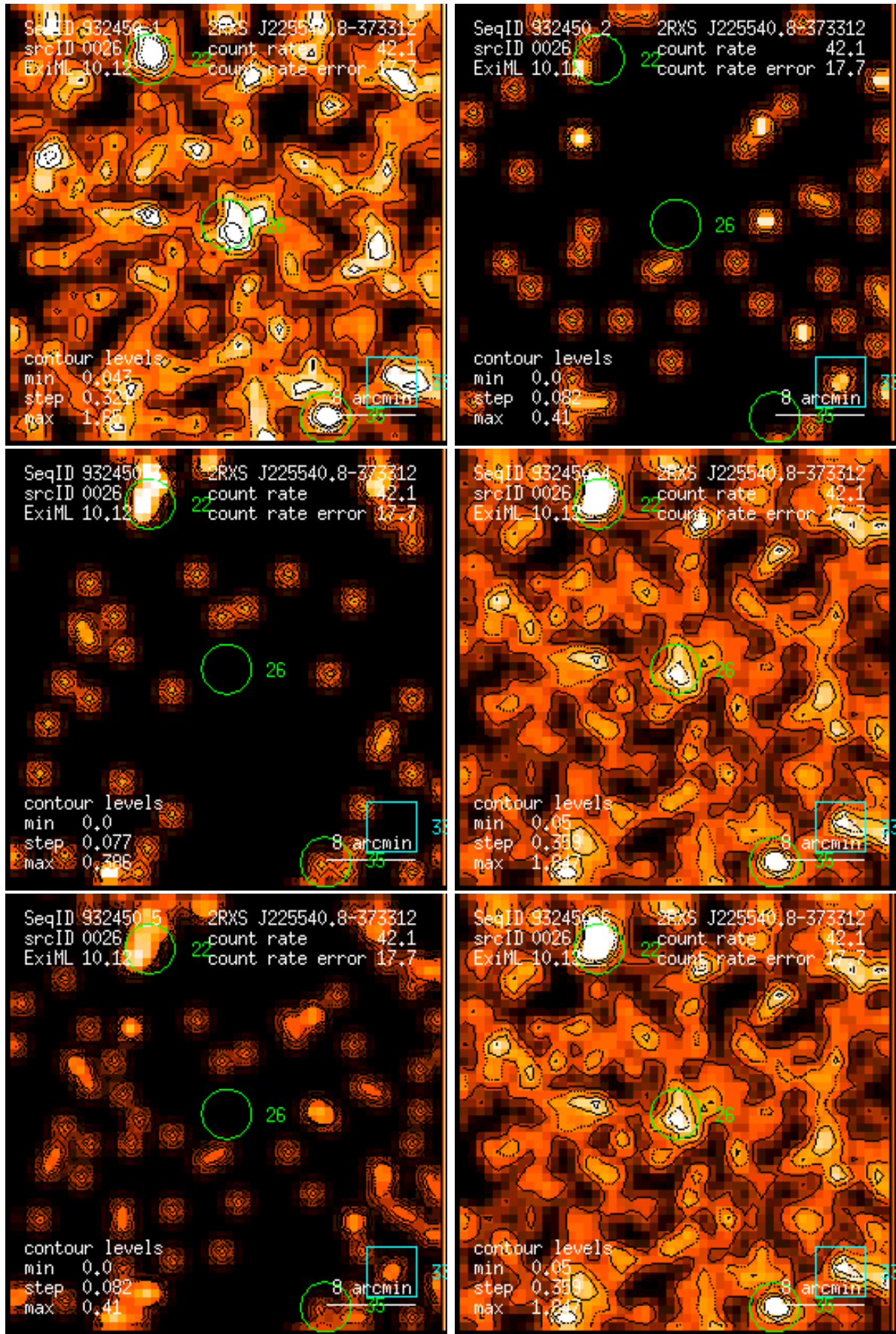
Figure 26: RASS 932450: detection 0026: band rate images, Gaussian filter: (1) PSPC channels 11 – 41, (2) 52 – 90, (3) 91 – 201, (4) 11 – 235, (5) 52 – 201, (6) 11 – 201. Broad band rates in counts/ks. Band rate contour levels in counts/ks/arcmin 2 .
