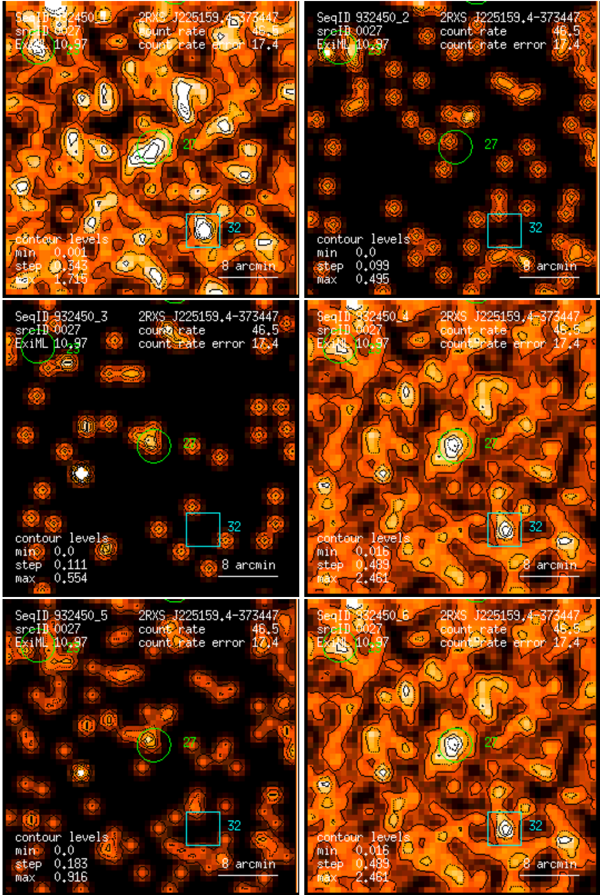
Figure 27: RASS 932450: detection 0027: band rate images, Gaussian filter: (1) PSPC channels 11 – 41, (2) 52 – 90, (3) 91 – 201, (4) 11 – 235, (5) 52 – 201, (6) 11 – 201. Broad band rates in counts/ks. Band rate contour levels in counts/ks/arcmin 2 .
