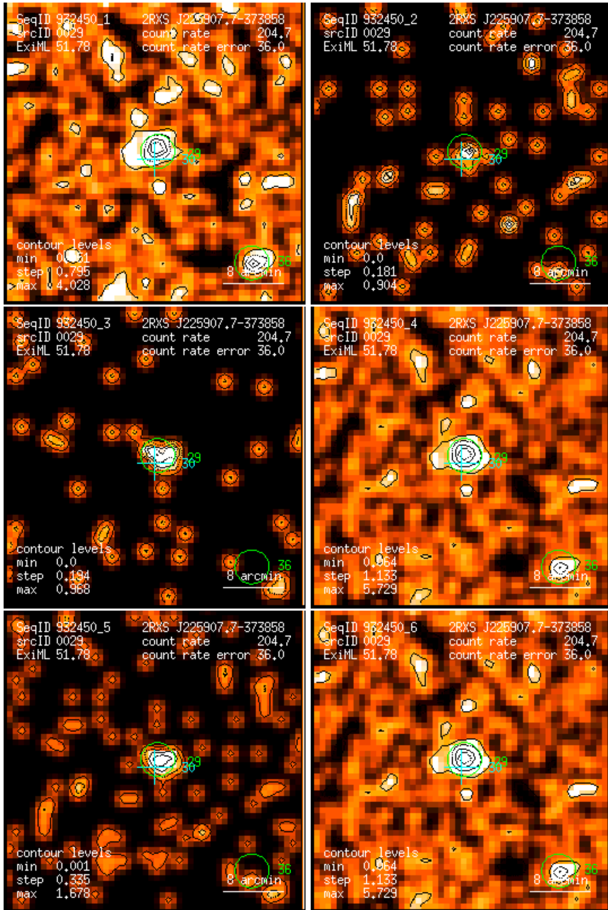
Figure 29: RASS 932450: detection 0029: band rate images, Gaussian filter: (1) PSPC channels 11 – 41, (2) 52 – 90, (3) 91 – 201, (4) 11 – 235, (5) 52 – 201, (6) 11 – 201. Broad band rates in counts/ks. Band rate contour levels in counts/ks/arcmin 2 .
