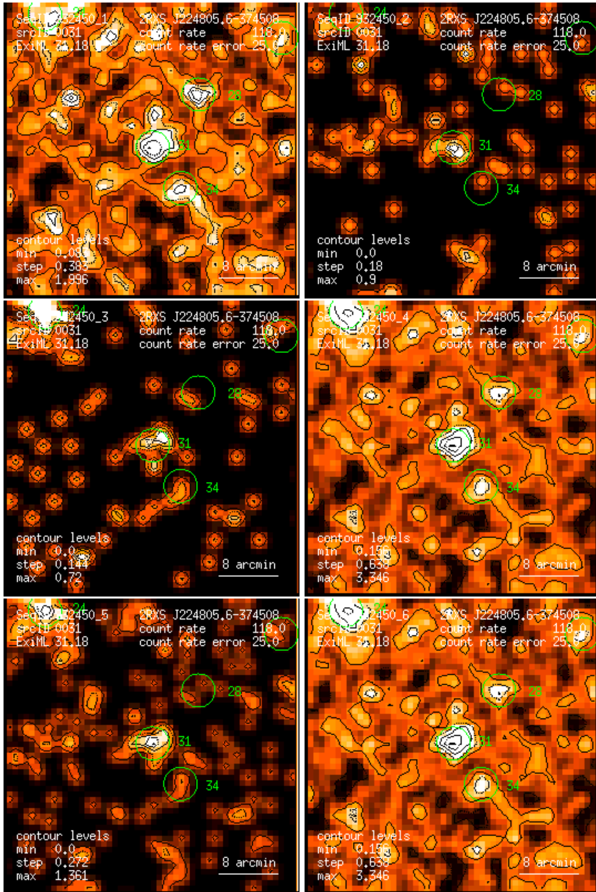
Figure 31: RASS 932450: detection 0031: band rate images, Gaussian filter: (1) PSPC channels 11 – 41, (2) 52 – 90, (3) 91 – 201, (4) 11 – 235, (5) 52 – 201, (6) 11 – 201. Broad band rates in counts/ks. Band rate contour levels in counts/ks/arcmin 2 .
