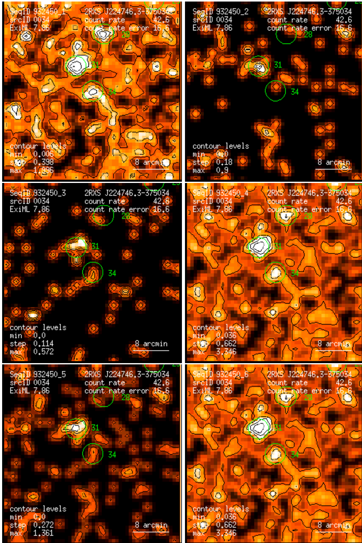
Figure 34: RASS 932450: detection 0034: band rate images, Gaussian filter: (1) PSPC channels 11 – 41, (2) 52 – 90, (3) 91 – 201, (4) 11 – 235, (5) 52 – 201, (6) 11 – 201. Broad band rates in counts/ks. Band rate contour levels in counts/ks/arcmin 2 .
