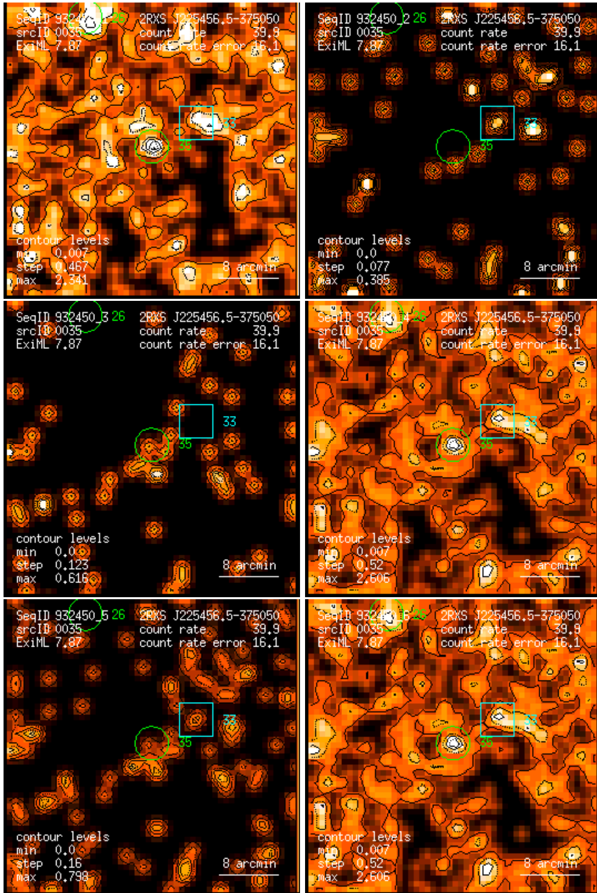
Figure 35: RASS 932450: detection 0035: band rate images, Gaussian filter: (1) PSPC channels 11 – 41, (2) 52 – 90, (3) 91 – 201, (4) 11 – 235, (5) 52 – 201, (6) 11 – 201. Broad band rates in counts/ks. Band rate contour levels in counts/ks/arcmin 2 .
