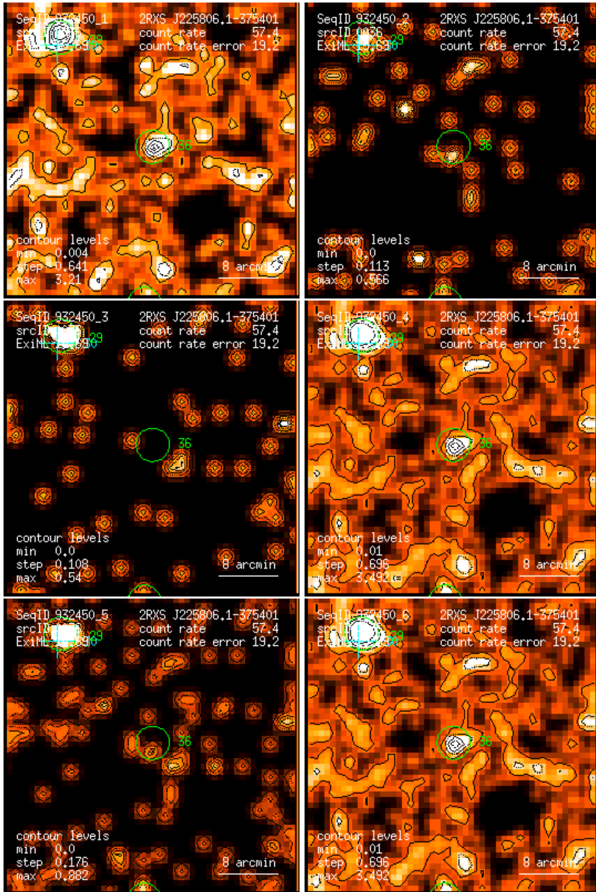
Figure 36: RASS 932450: detection 0036: band rate images, Gaussian filter: (1) PSPC channels 11 – 41, (2) 52 – 90, (3) 91 – 201, (4) 11 – 235, (5) 52 – 201, (6) 11 – 201. Broad band rates in counts/ks. Band rate contour levels in counts/ks/arcmin 2 .
