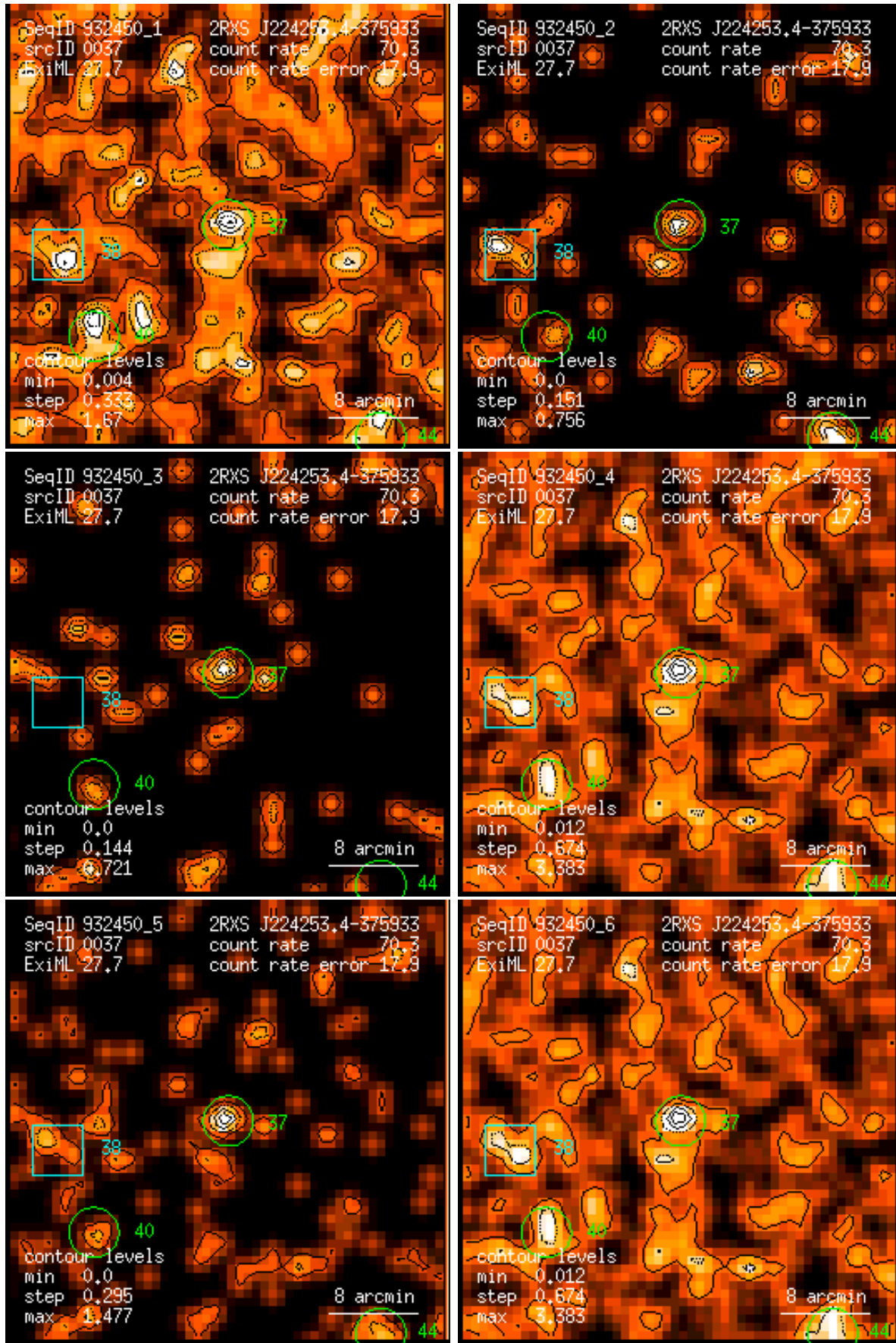
Figure 37: RASS 932450: detection 0037: band rate images, Gaussian filter: (1) PSPC channels 11 – 41, (2) 52 – 90, (3) 91 – 201, (4) 11 – 235, (5) 52 – 201, (6) 11 – 201. Broad band rates in counts/ks. Band rate contour levels in counts/ks/arcmin 2 .
