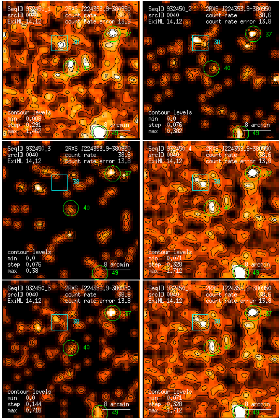
Figure 40: RASS 932450: detection 0040: band rate images, Gaussian filter: (1) PSPC channels 11 – 41, (2) 52 – 90, (3) 91 – 201, (4) 11 – 235, (5) 52 – 201, (6) 11 – 201. Broad band rates in counts/ks. Band rate contour levels in counts/ks/arcmin 2 .
