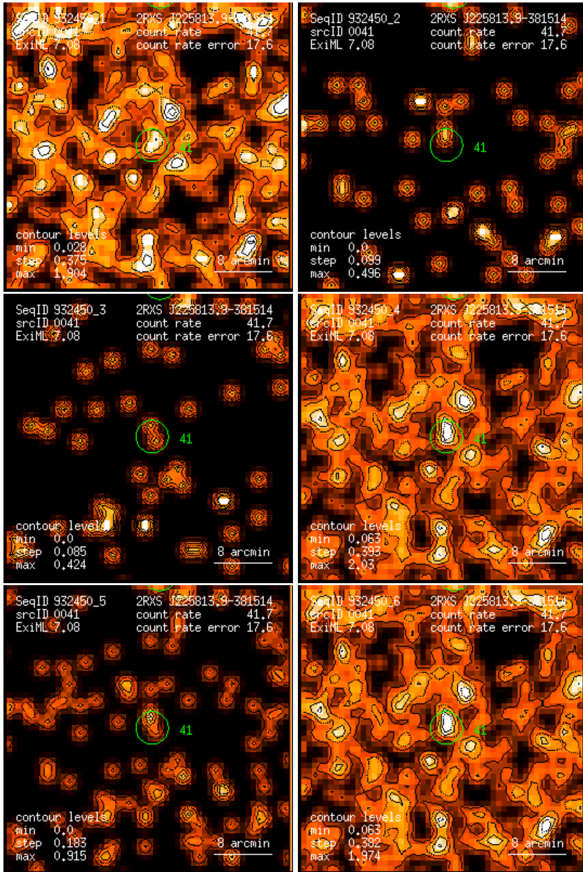
Figure 41: RASS 932450: detection 0041: band rate images, Gaussian filter: (1) PSPC channels 11 – 41, (2) 52 – 90, (3) 91 – 201, (4) 11 – 235, (5) 52 – 201, (6) 11 – 201. Broad band rates in counts/ks. Band rate contour levels in counts/ks/arcmin 2 .
