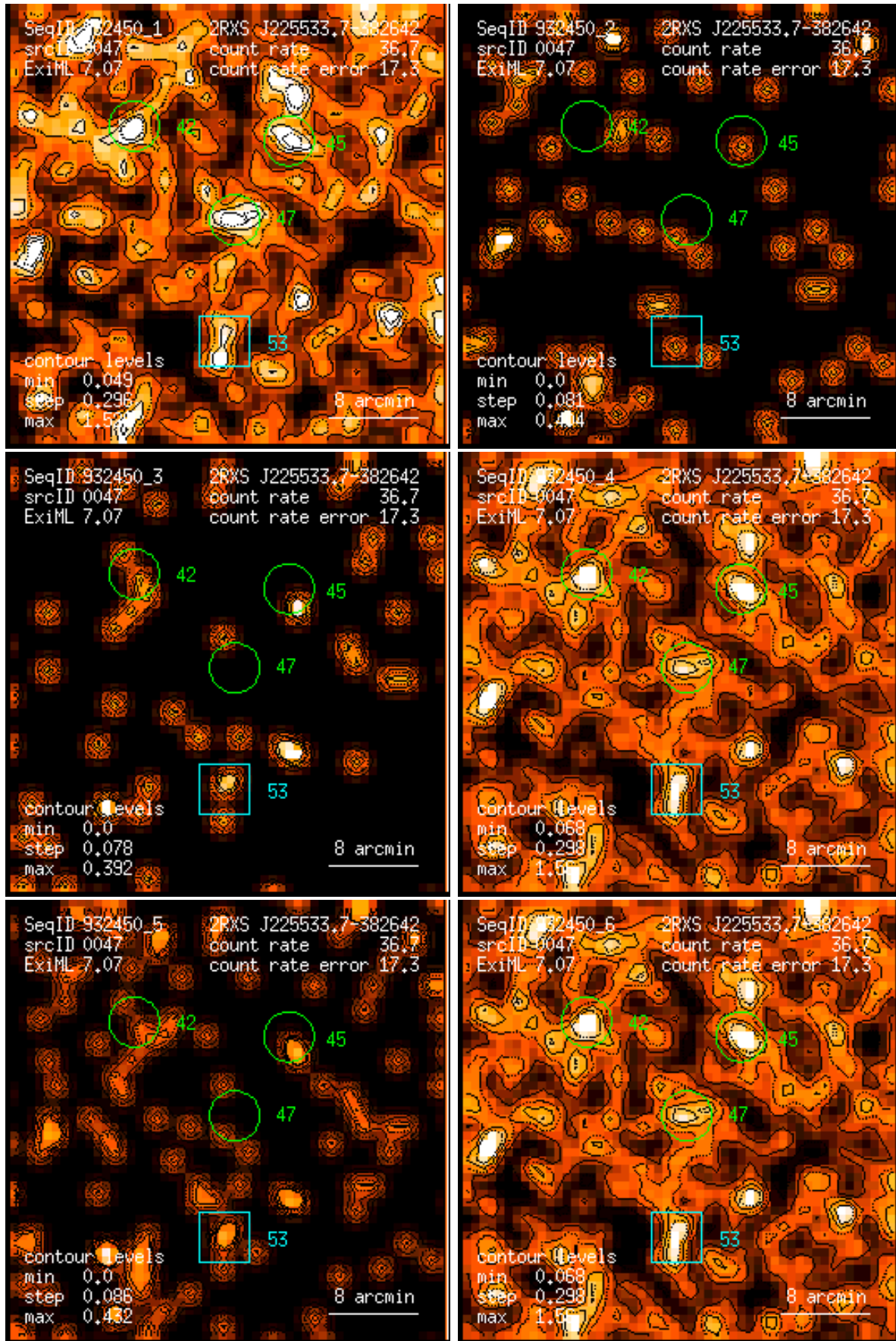
Figure 47: RASS 932450: detection 0047: band rate images, Gaussian filter: (1) PSPC channels 11 – 41, (2) 52 – 90, (3) 91 – 201, (4) 11 – 235, (5) 52 – 201, (6) 11 – 201. Broad band rates in counts/ks. Band rate contour levels in counts/ks/arcmin 2 .
