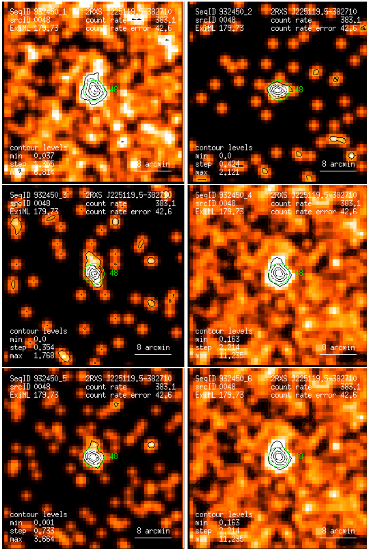
Figure 48: RASS 932450: detection 0048: band rate images, Gaussian filter: (1) PSPC channels 11 – 41, (2) 52 – 90, (3) 91 – 201, (4) 11 – 235, (5) 52 – 201, (6) 11 – 201. Broad band rates in counts/ks. Band rate contour levels in counts/ks/arcmin 2 .
