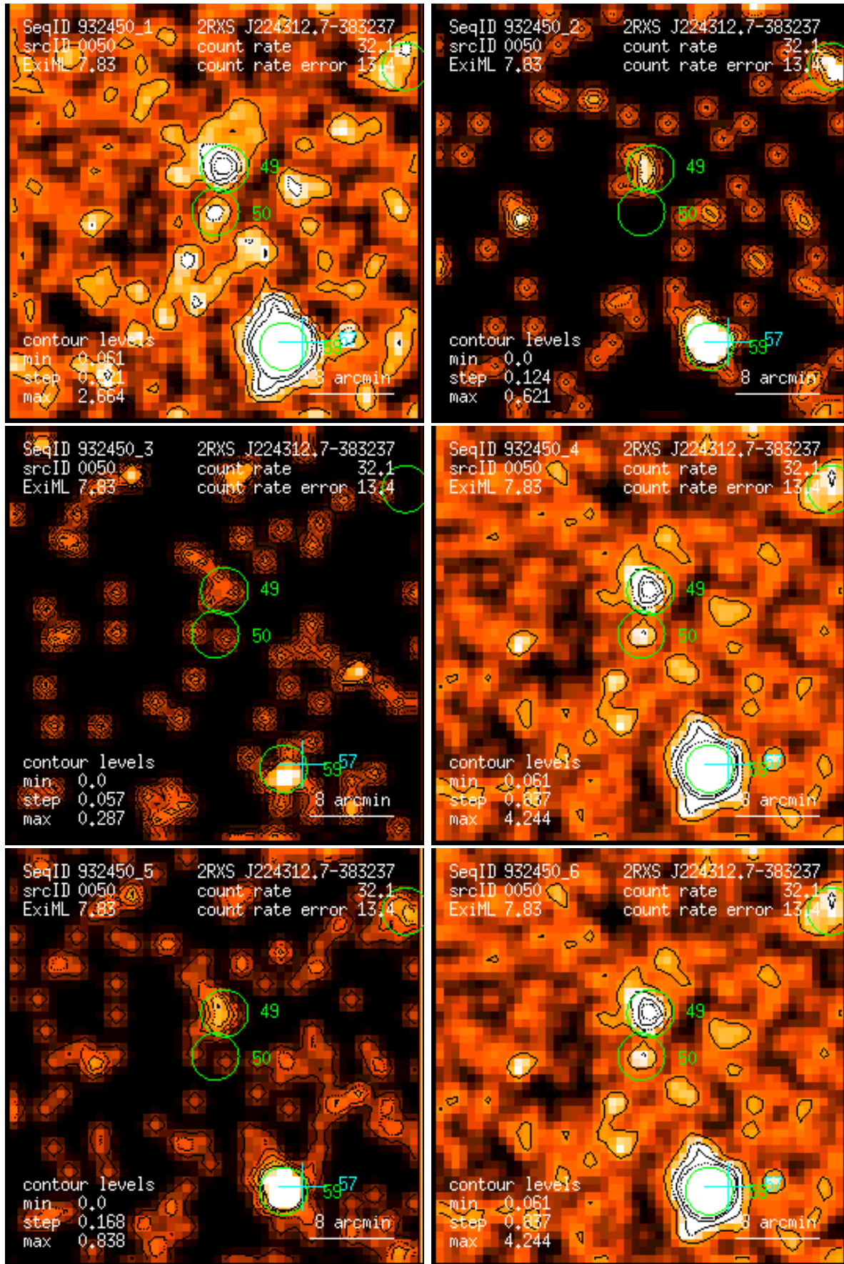
Figure 50: RASS 932450: detection 0050: band rate images, Gaussian filter: (1) PSPC channels 11 – 41, (2) 52 – 90, (3) 91 – 201, (4) 11 – 235, (5) 52 – 201, (6) 11 – 201. Broad band rates in counts/ks. Band rate contour levels in counts/ks/arcmin 2 .
