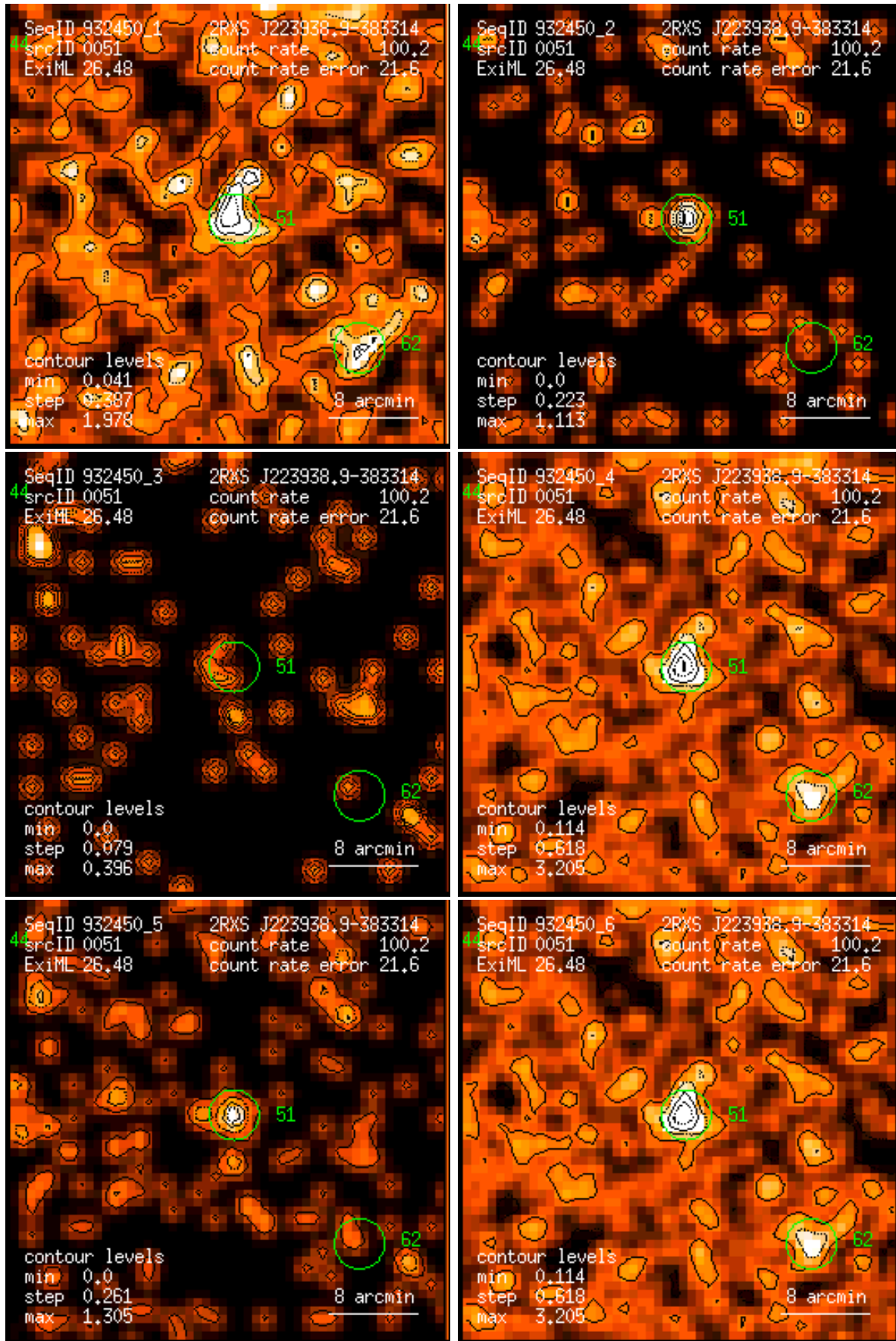
Figure 51: RASS 932450: detection 0051: band rate images, Gaussian filter: (1) PSPC channels 11 – 41, (2) 52 – 90, (3) 91 – 201, (4) 11 – 235, (5) 52 – 201, (6) 11 – 201. Broad band rates in counts/ks. Band rate contour levels in counts/ks/arcmin 2 .
