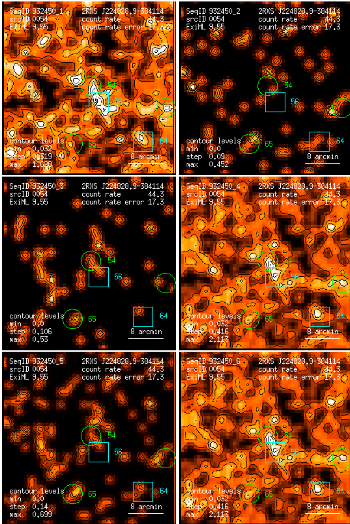
Figure 54: RASS 932450: detection 0054: band rate images, Gaussian filter: (1) PSPC channels 11 – 41, (2) 52 – 90, (3) 91 – 201, (4) 11 – 235, (5) 52 – 201, (6) 11 – 201. Broad band rates in counts/ks. Band rate contour levels in counts/ks/arcmin 2 .
