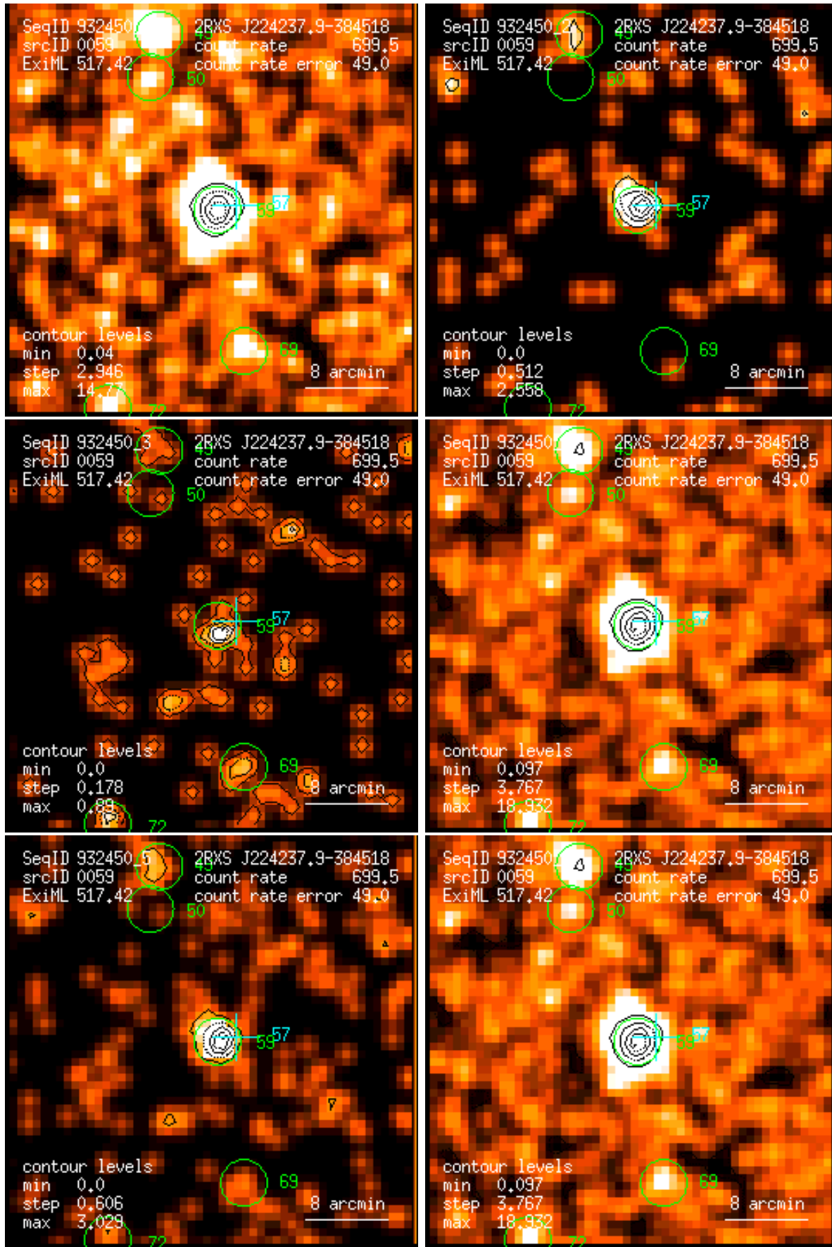
Figure 59: RASS 932450: detection 0059: band rate images, Gaussian filter: (1) PSPC channels 11 – 41, (2) 52 – 90, (3) 91 – 201, (4) 11 – 235, (5) 52 – 201, (6) 11 – 201. Broad band rates in counts/ks. Band rate contour levels in counts/ks/arcmin 2 .
