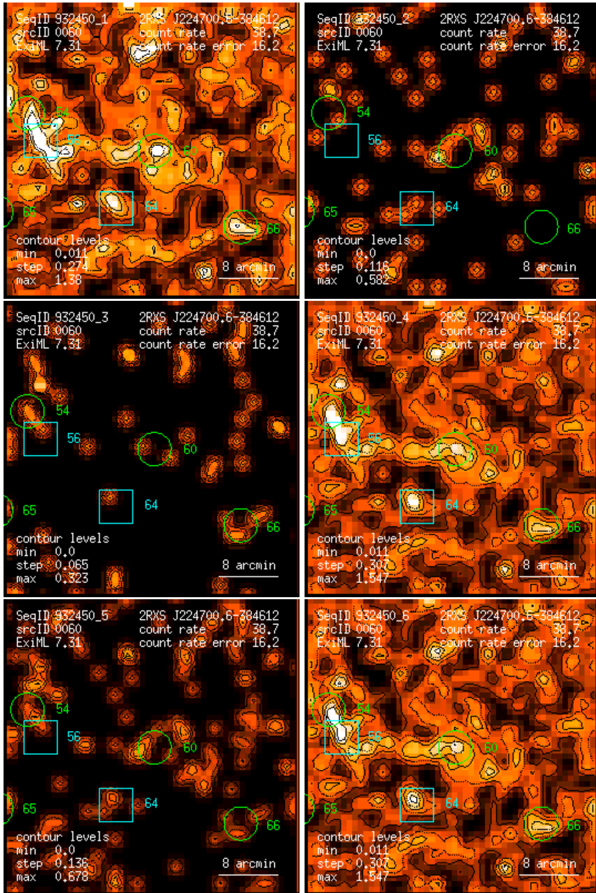
Figure 60: RASS 932450: detection 0060: band rate images, Gaussian filter: (1) PSPC channels 11 – 41, (2) 52 – 90, (3) 91 – 201, (4) 11 – 235, (5) 52 – 201, (6) 11 – 201. Broad band rates in counts/ks. Band rate contour levels in counts/ks/arcmin 2 .
