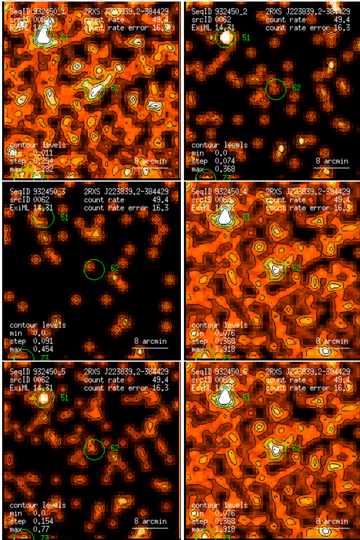
Figure 62: RASS 932450: detection 0062: band rate images, Gaussian filter: (1) PSPC channels 11 – 41, (2) 52 – 90, (3) 91 – 201, (4) 11 – 235, (5) 52 – 201, (6) 11 – 201. Broad band rates in counts/ks. Band rate contour levels in counts/ks/arcmin 2 .
