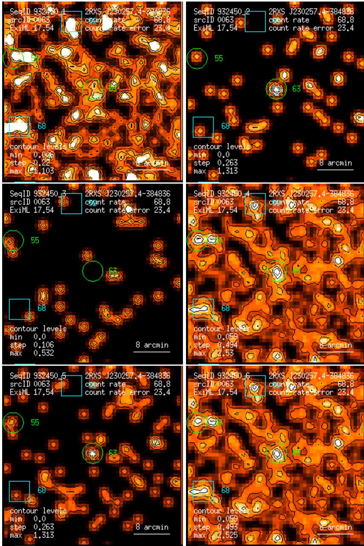
Figure 63: RASS 932450: detection 0063: band rate images, Gaussian filter: (1) PSPC channels 11 – 41, (2) 52 – 90, (3) 91 – 201, (4) 11 – 235, (5) 52 – 201, (6) 11 – 201. Broad band rates in counts/ks. Band rate contour levels in counts/ks/arcmin 2 .
