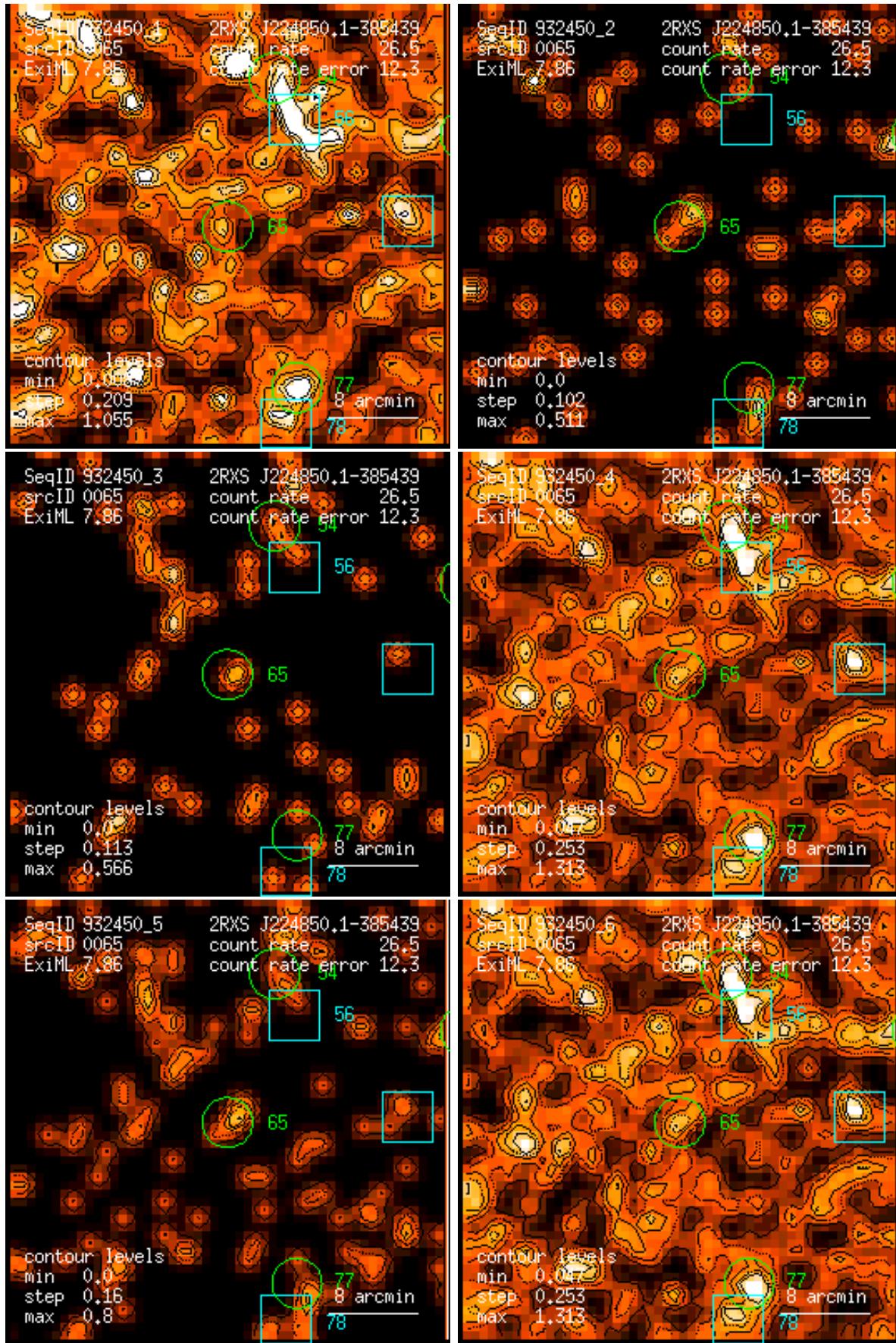
Figure 65: RASS 932450: detection 0065: band rate images, Gaussian filter: (1) PSPC channels 11 – 41, (2) 52 – 90, (3) 91 – 201, (4) 11 – 235, (5) 52 – 201, (6) 11 – 201. Broad band rates in counts/ks. Band rate contour levels in counts/ks/arcmin 2 .
