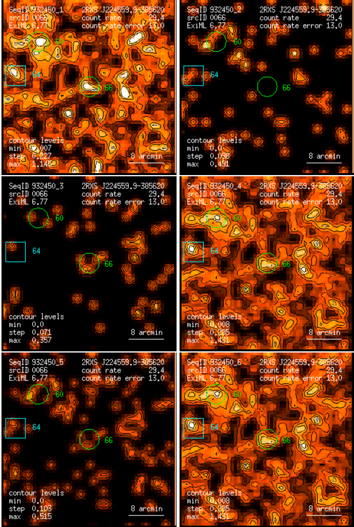
Figure 66: RASS 932450: detection 0066: band rate images, Gaussian filter: (1) PSPC channels 11 – 41, (2) 52 – 90, (3) 91 – 201, (4) 11 – 235, (5) 52 – 201, (6) 11 – 201. Broad band rates in counts/ks. Band rate contour levels in counts/ks/arcmin 2 .
