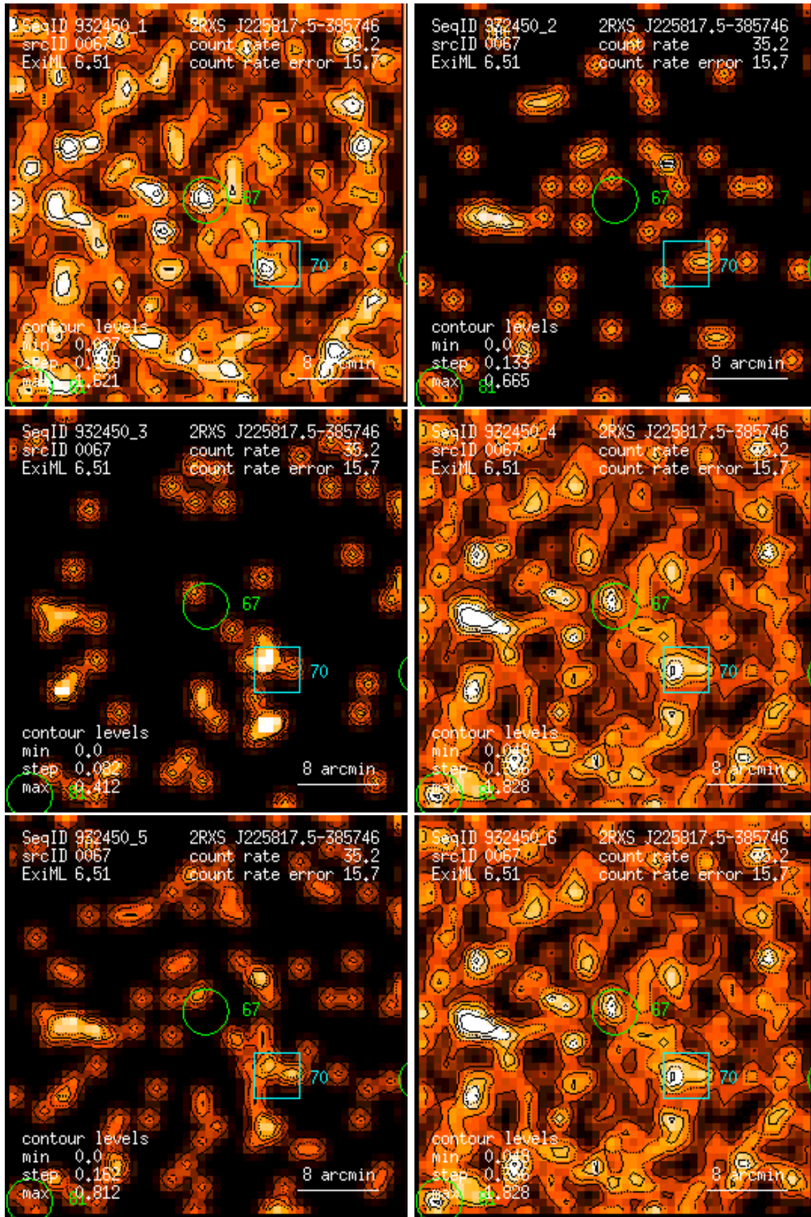
Figure 67: RASS 932450: detection 0067: band rate images, Gaussian filter: (1) PSPC channels 11 – 41, (2) 52 – 90, (3) 91 – 201, (4) 11 – 235, (5) 52 – 201, (6) 11 – 201. Broad band rates in counts/ks. Band rate contour levels in counts/ks/arcmin 2 .
