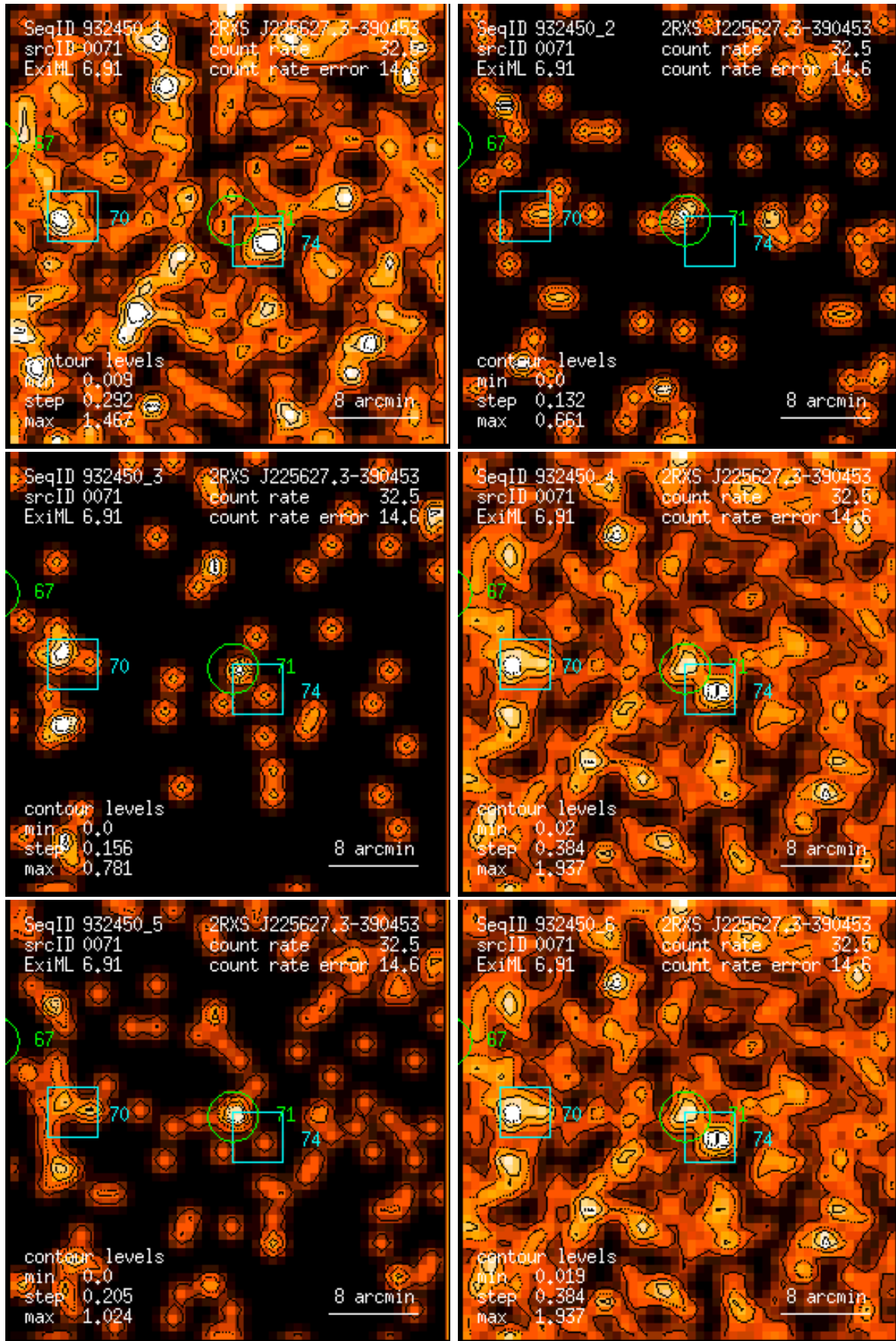
Figure 71: RASS 932450: detection 0071: band rate images, Gaussian filter: (1) PSPC channels 11 – 41, (2) 52 – 90, (3) 91 – 201, (4) 11 – 235, (5) 52 – 201, (6) 11 – 201. Broad band rates in counts/ks. Band rate contour levels in counts/ks/arcmin 2 .
