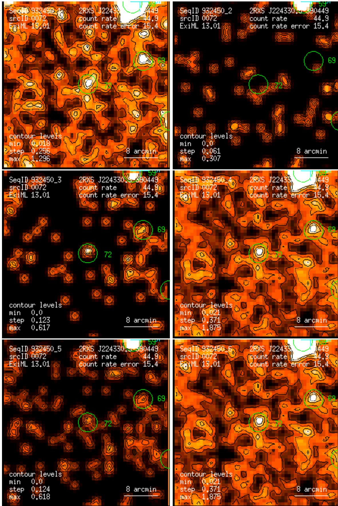
Figure 72: RASS 932450: detection 0072: band rate images, Gaussian filter: (1) PSPC channels 11 – 41, (2) 52 – 90, (3) 91 – 201, (4) 11 – 235, (5) 52 – 201, (6) 11 – 201. Broad band rates in counts/ks. Band rate contour levels in counts/ks/arcmin 2 .
